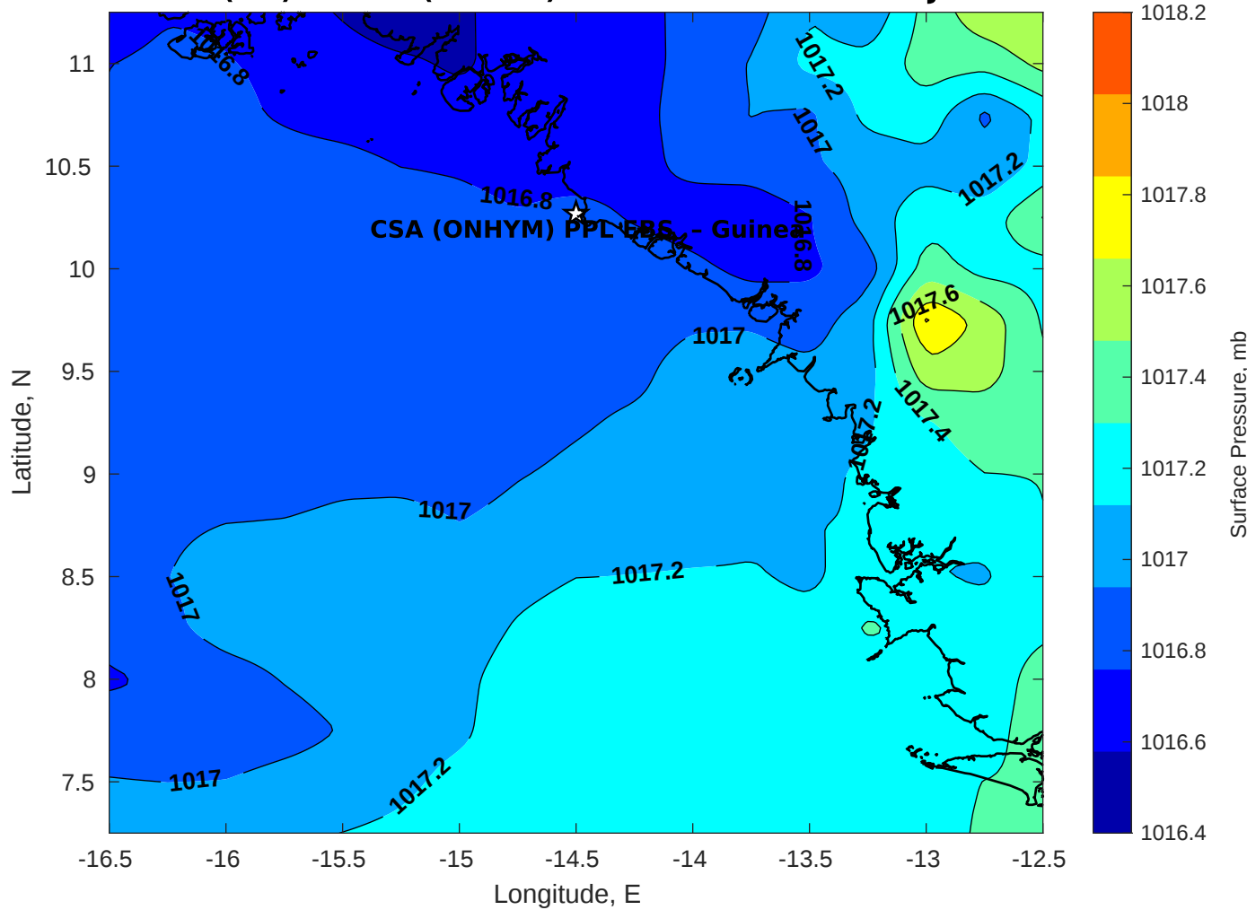
Surface Pressure (mb) for CSA (ONHYM) PPL EBS - Guinea at 27-Jul-2025 12:00:00
