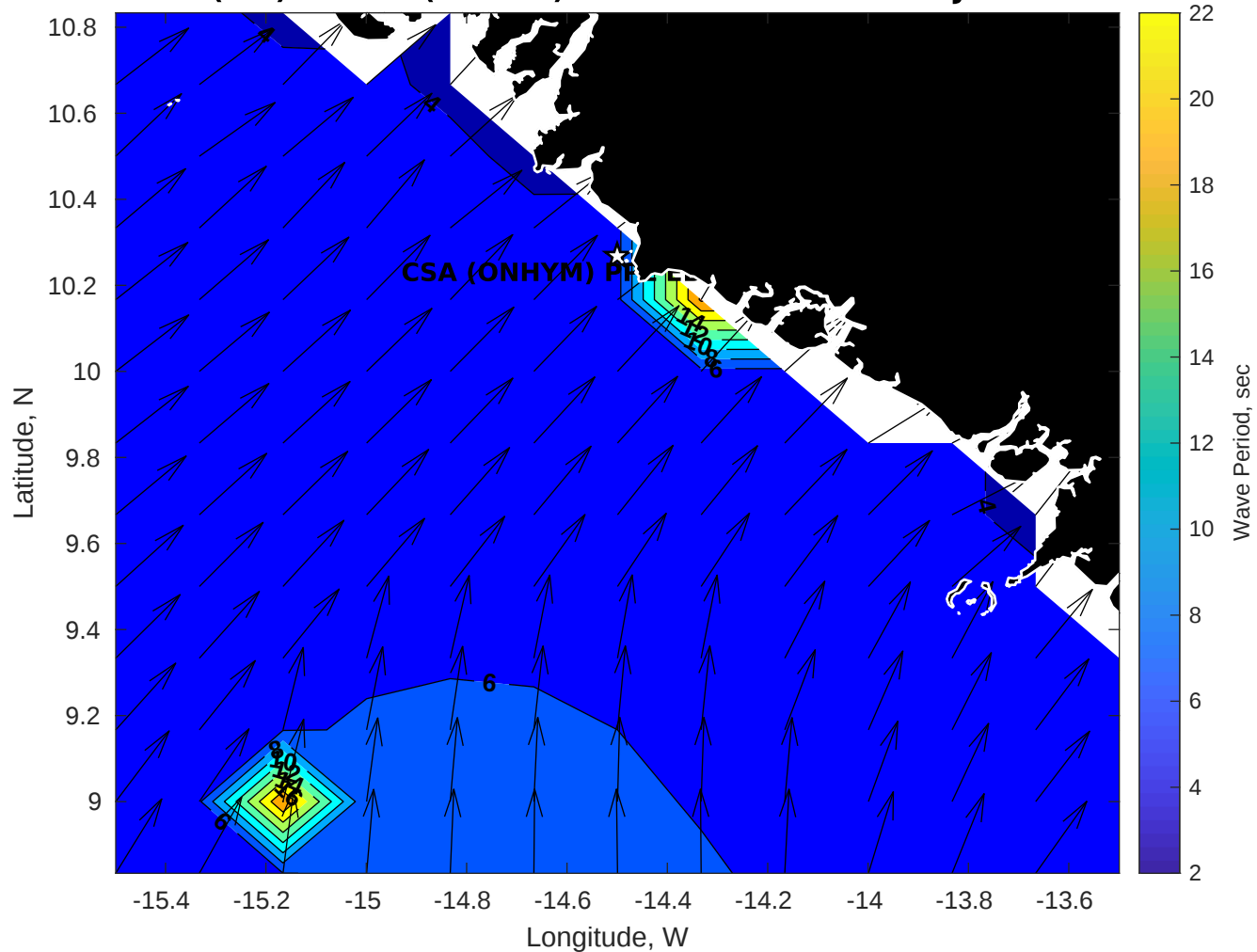
Wave Period (sec) for CSA (ONHYM) PPL EBS - Guinea at 25-Jul-2025 21:00:00
