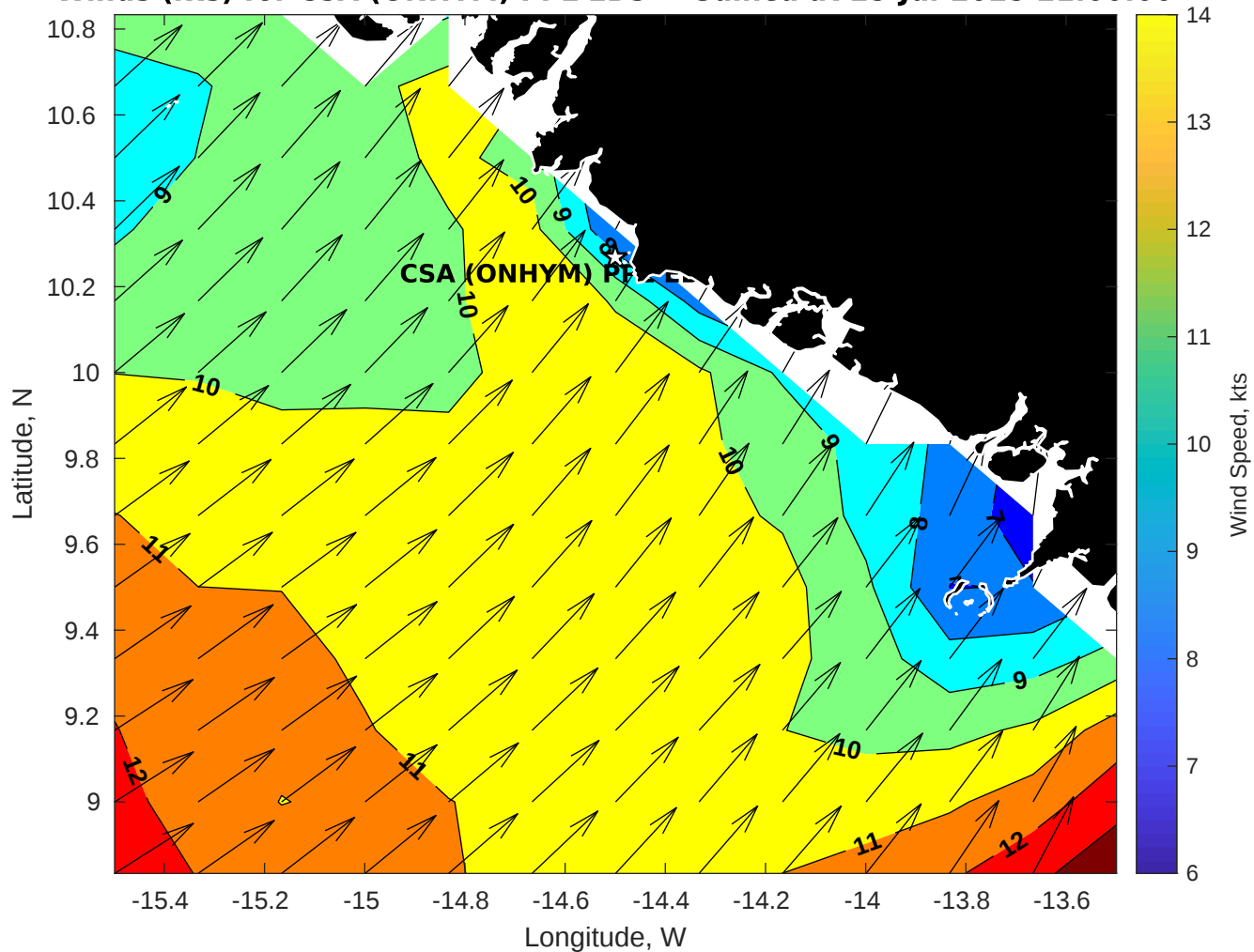
Winds (kts) for CSA (ONHYM) PPL EBS - Guinea at 25-Jul-2025 21:00:00
