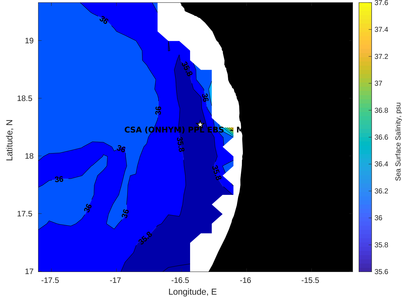
Surface Salinity for CSA (ONHYM) PPL EBS - Mauritania at 25-Jul-2025 00:00:00
