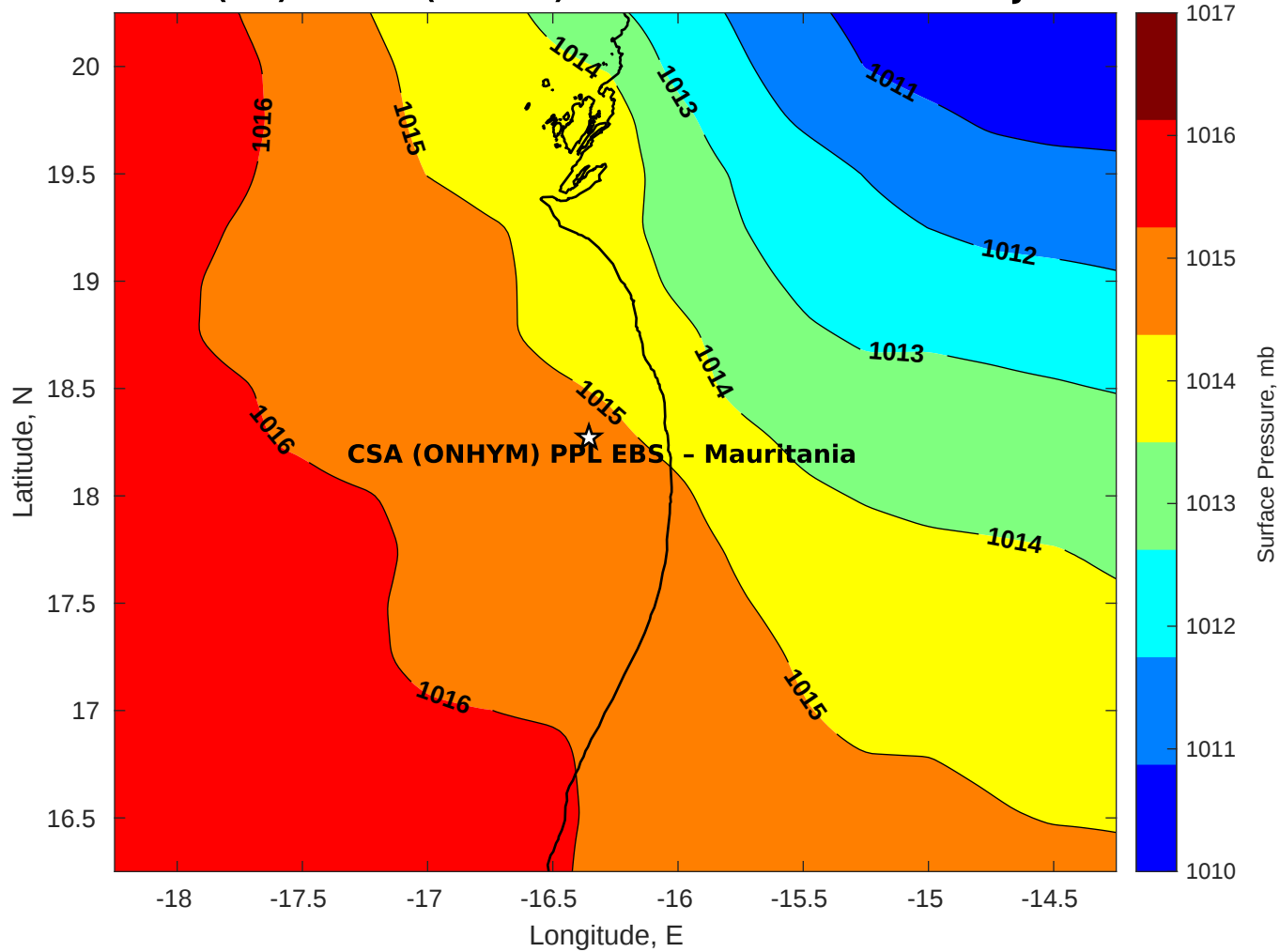
Surface Pressure (mb) for CSA (ONHYM) PPL EBS - Mauritania at 27-Jul-2025 12:00:00
