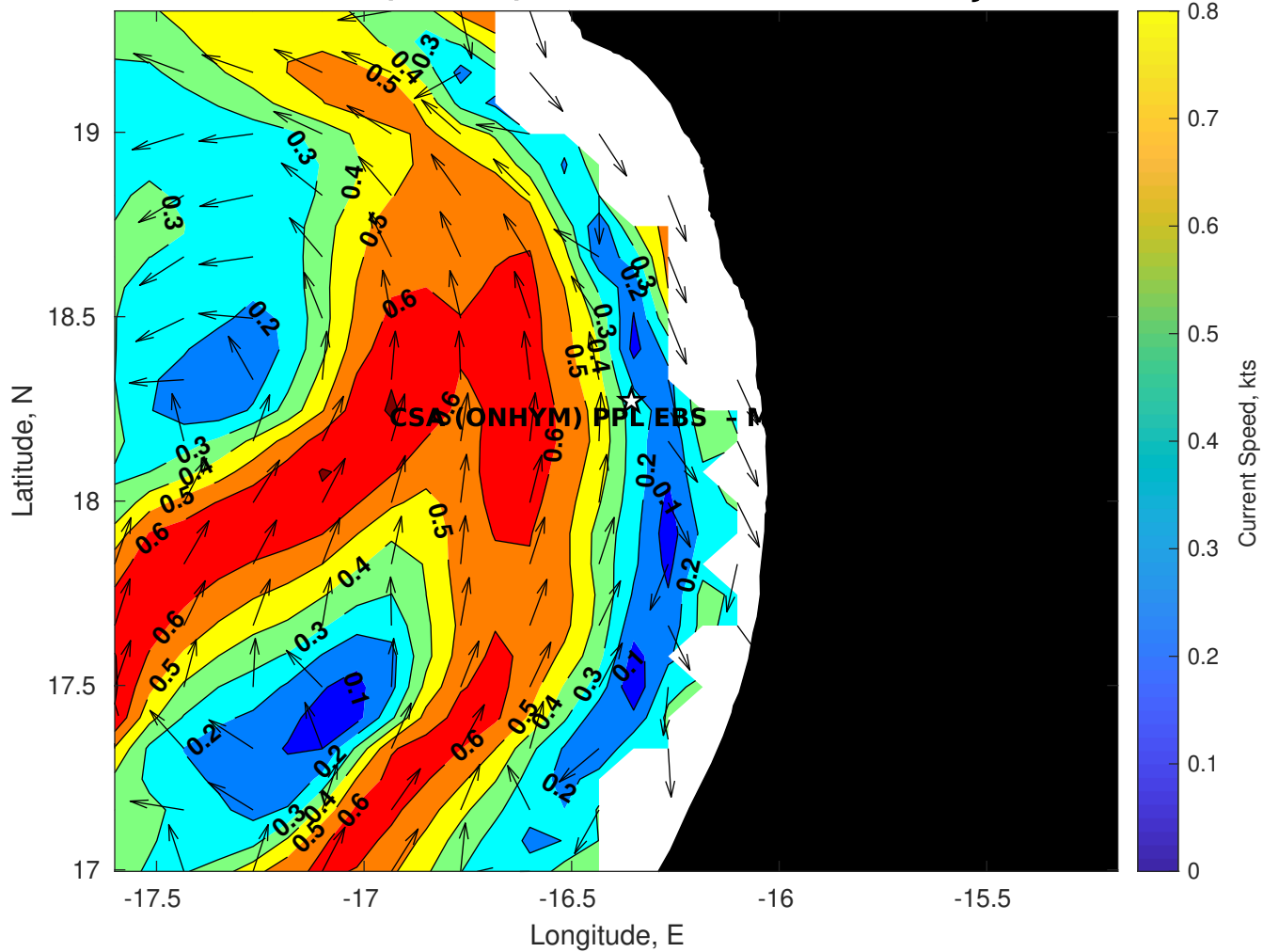
Surface Currents for CSA (ONHYM) PPL EBS - Mauritania at 25-Jul-2025 00:00:00
