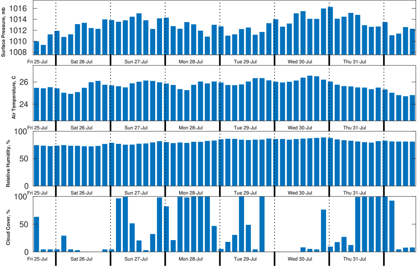
Met Forecast for CSA (ONHYM) PPL EBS - Mauritania from 25-Jul-2025 12:00:00 to 01-Aug-2025 12:00:00
