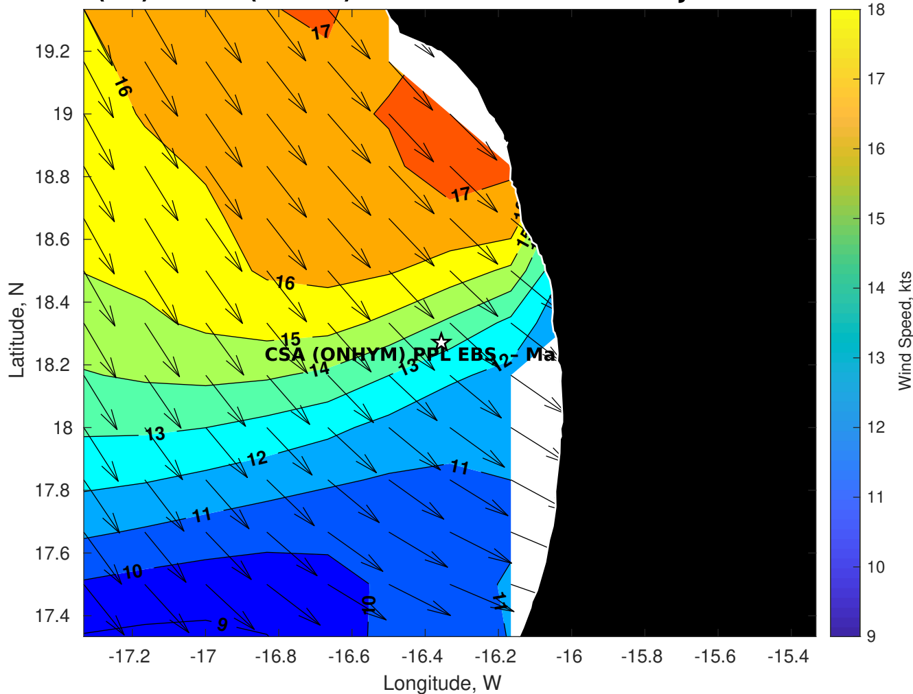
Winds (kts) for CSA (ONHYM) PPL EBS - Mauritania at 25-Jul-2025 21:00:00
