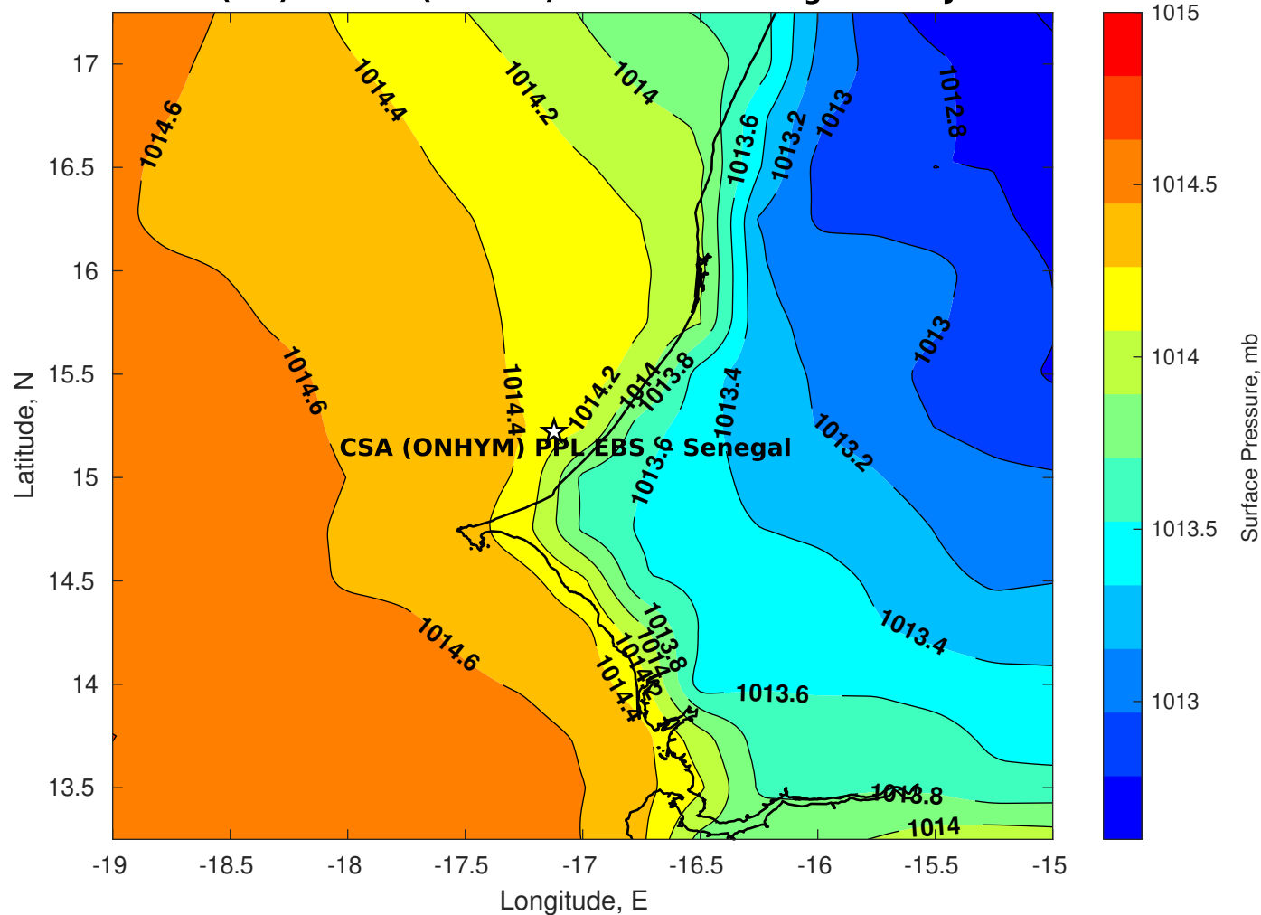
Surface Pressure (mb) for CSA (ONHYM) PPL EBS - Senegal at 26-Jul-2025 12:00:00
