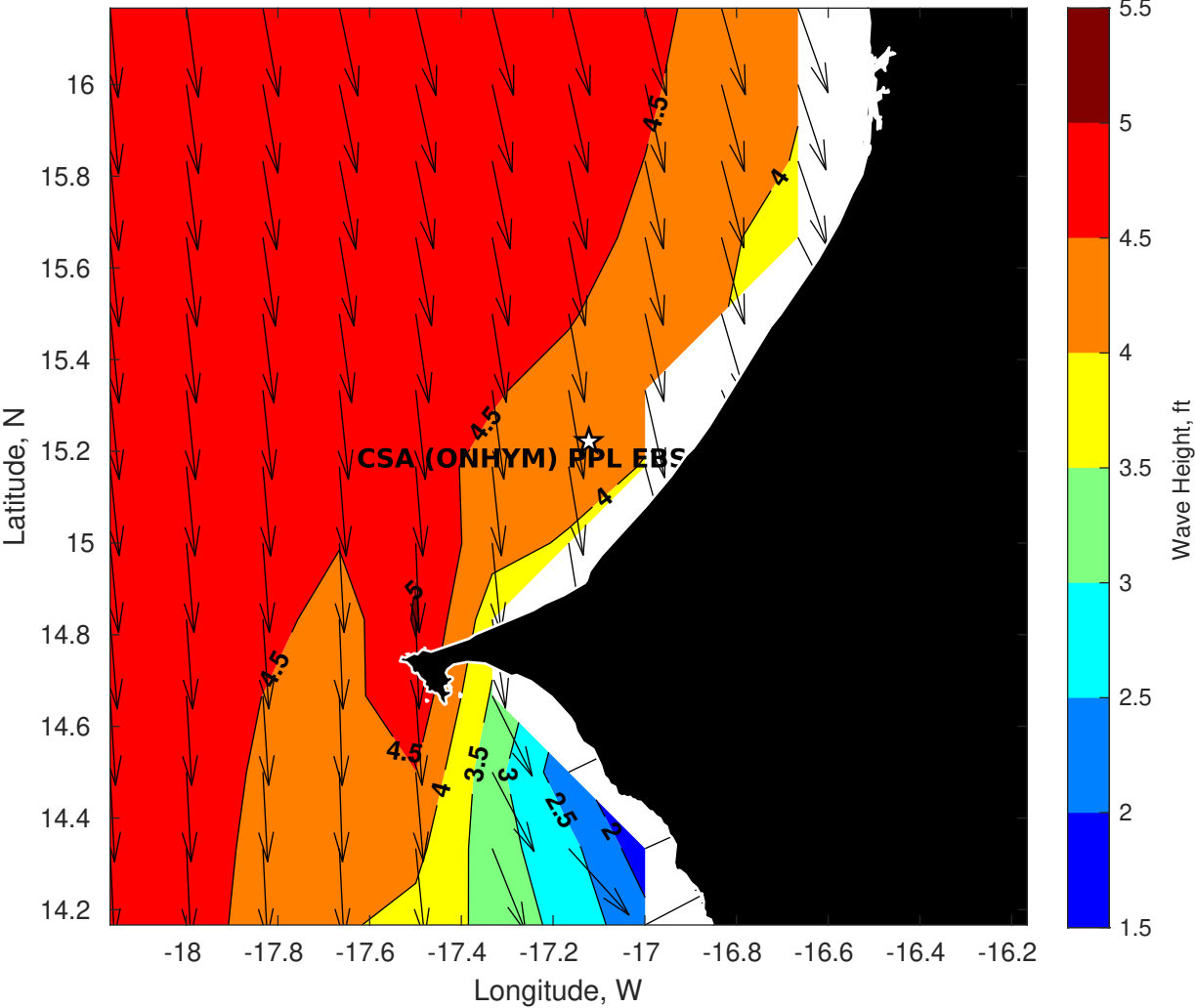
Wave Height (ft) for CSA (ONHYM) PPL EBS - Senegal at 25-Jul-2025 21:00:00
