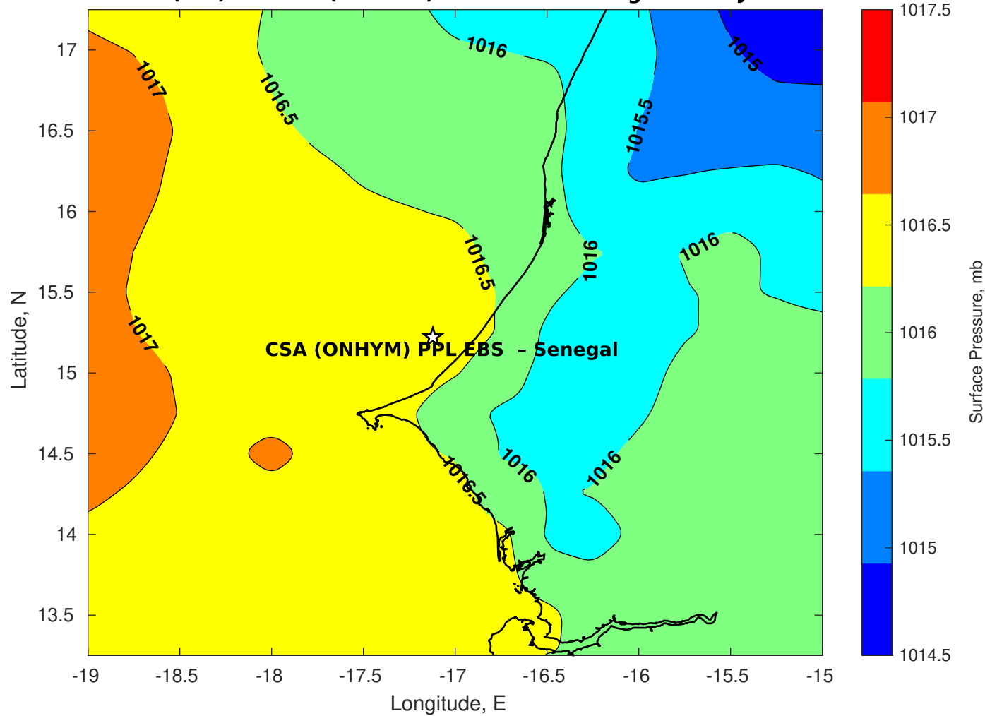
Surface Pressure (mb) for CSA (ONHYM) PPL EBS - Senegal at 27-Jul-2025 12:00:00
