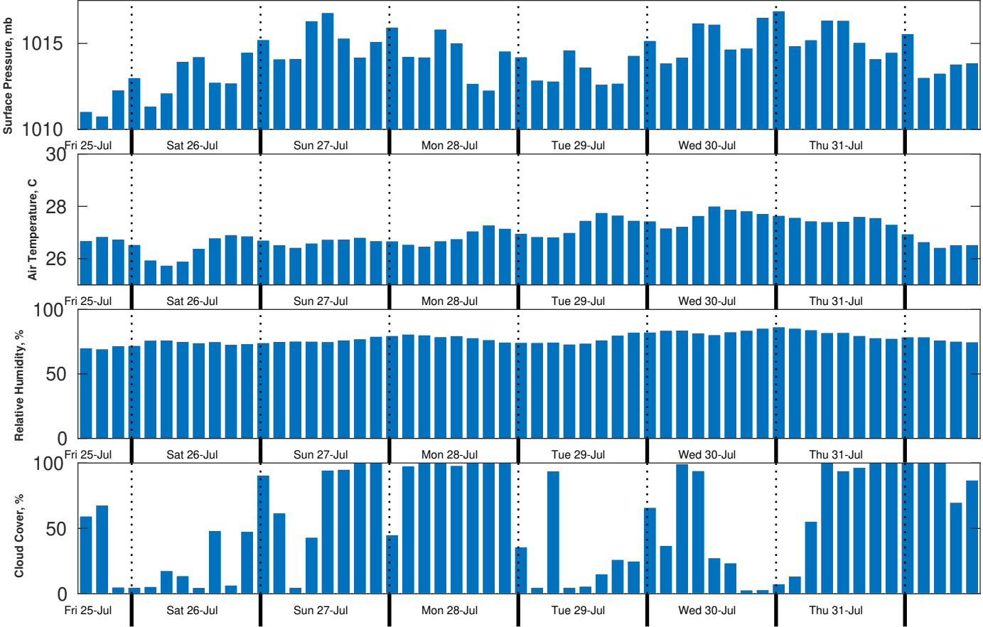
Met Forecast for CSA (ONHYM) PPL EBS - Senegal from 25-Jul-2025 12:00:00 to 01-Aug-2025 12:00:00
