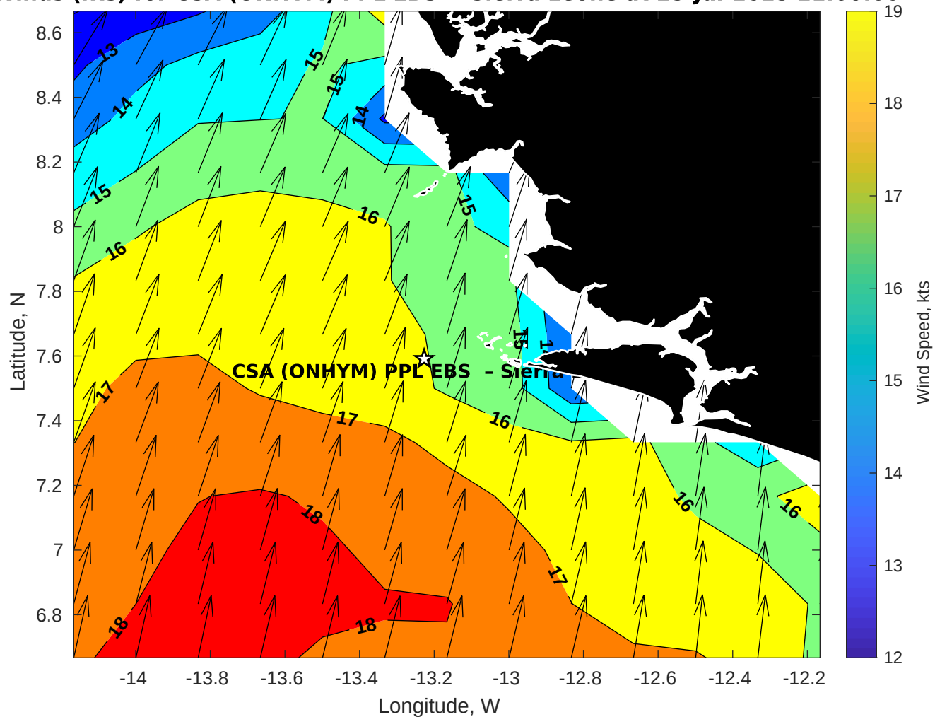
Winds (kts) for CSA (ONHYM) PPL EBS - Sierra Leone at 25-Jul-2025 21:00:00
