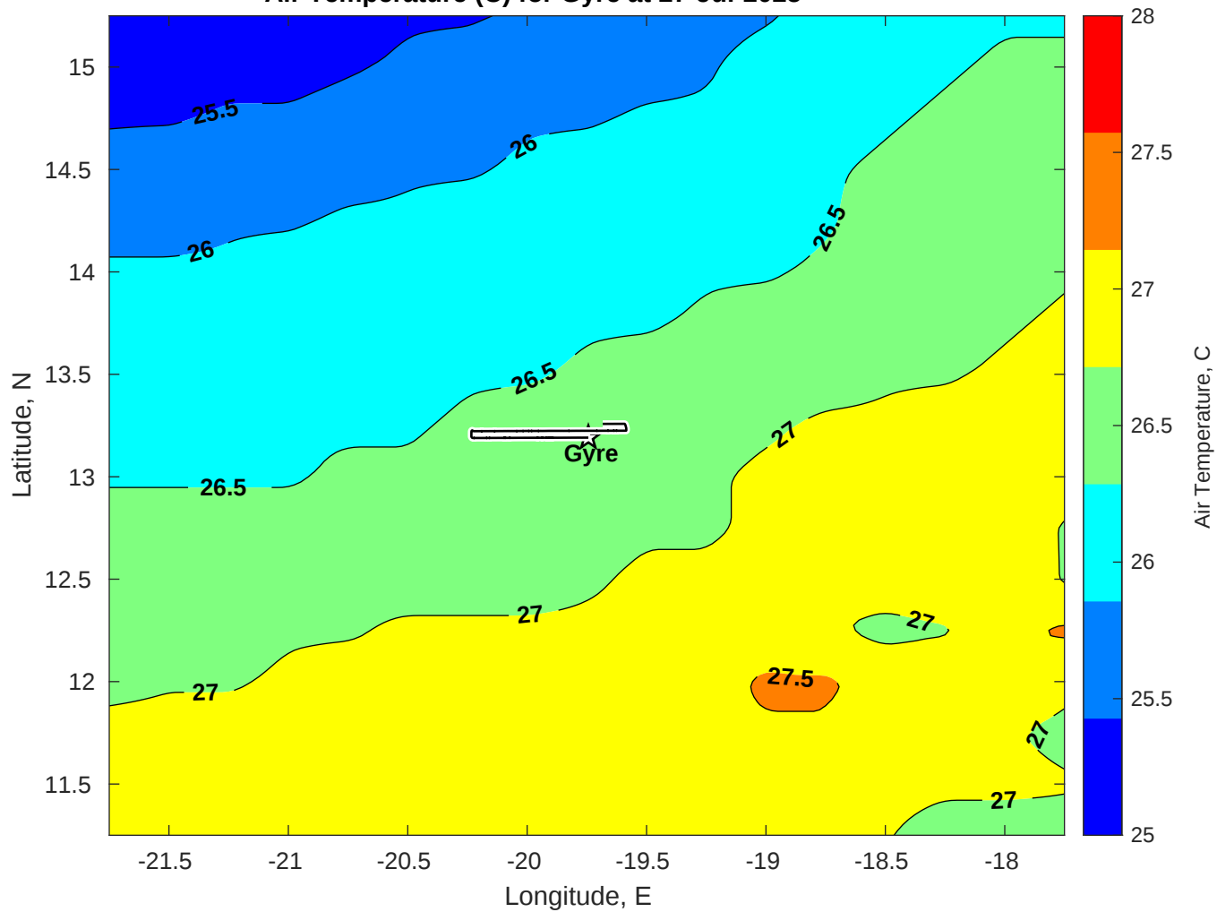
Air Temperature (C) for Gyre at 27-Jul-2025
