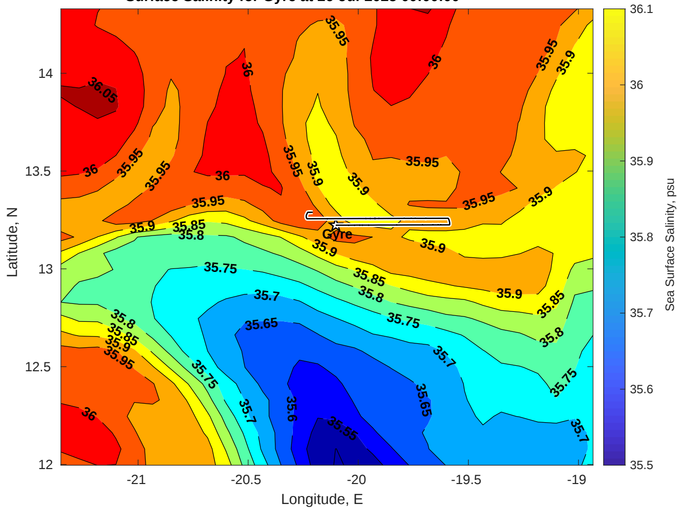
Surface Salinity for Gyre at 26-Jul-2025 00:00:00
