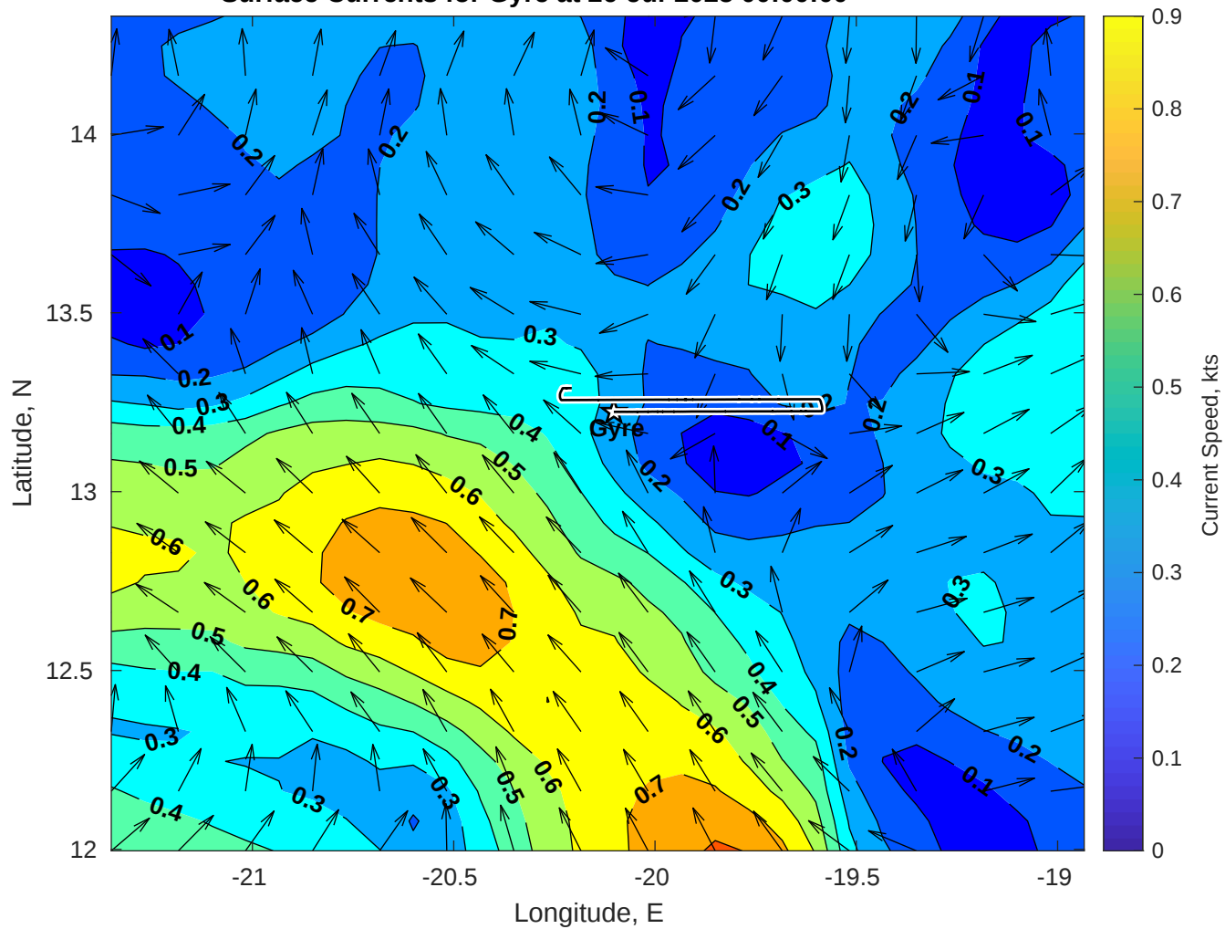
Surface Currents for Gyre at 26-Jul-2025 00:00:00
