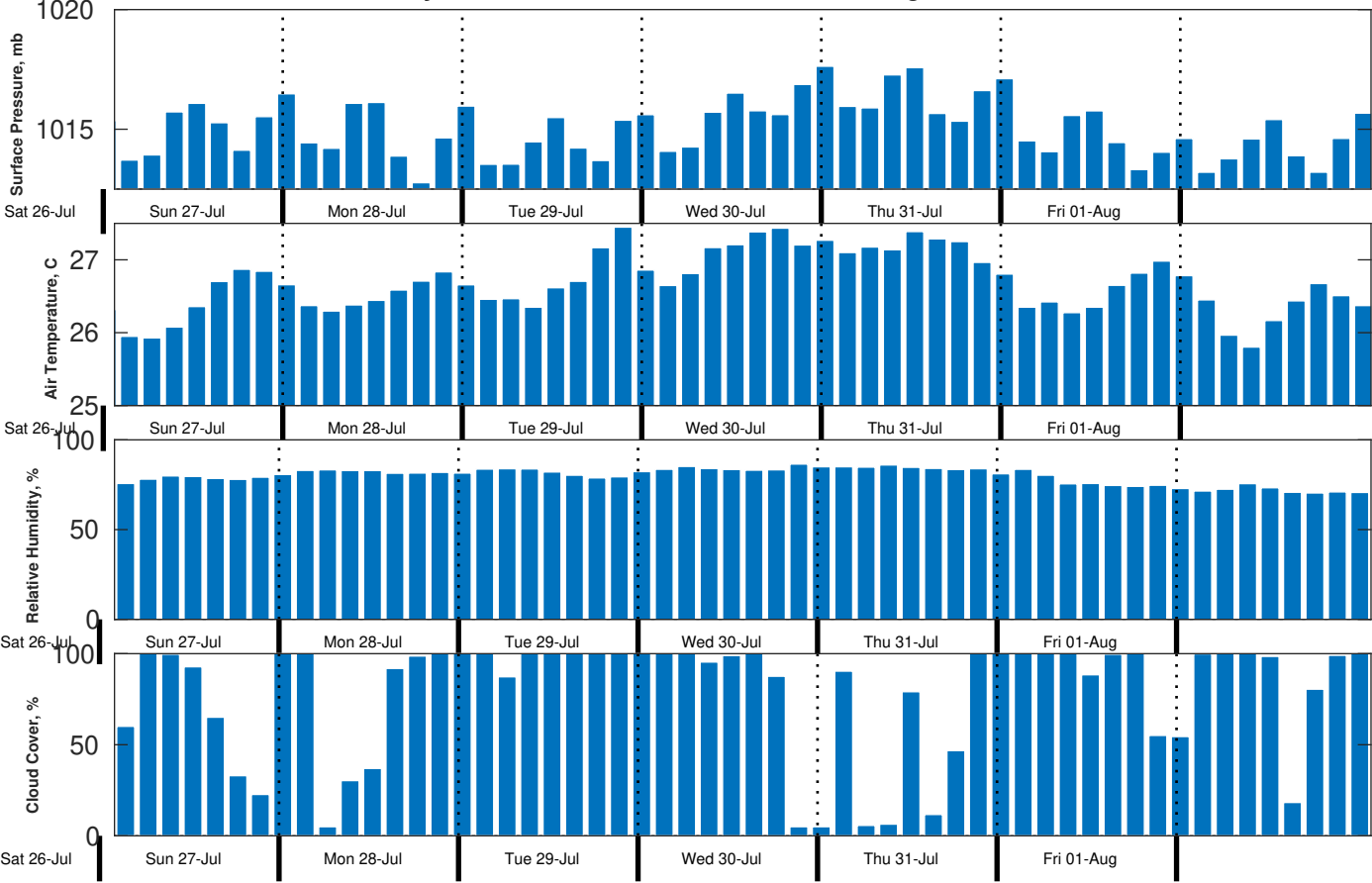
Met Forecast for Gyre from 26-Jul-2025 23:00:00 to 02-Aug-2025 23:00:00
