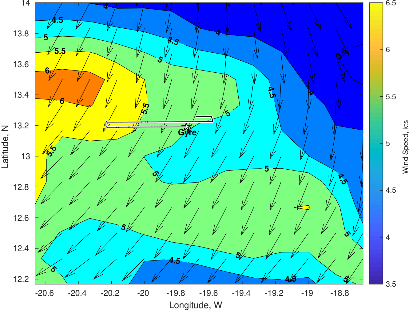
Winds (kts) for Gyre at 27-Jul-2025 09:00:00
