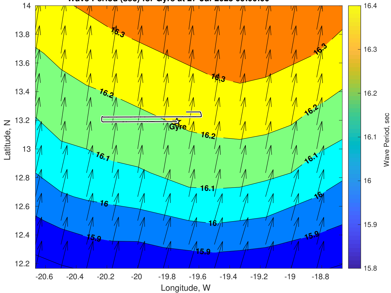
Wave Period (sec) for Gyre at 27-Jul-2025 09:00:00
