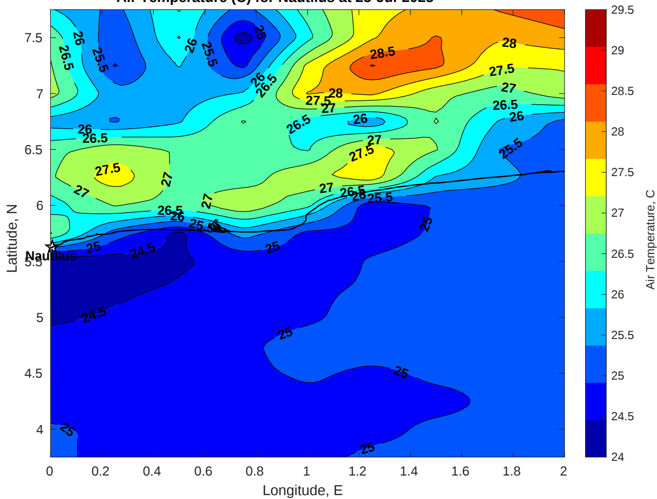
Air Temperature (C) for Nautilus at 25-Jul-2025
