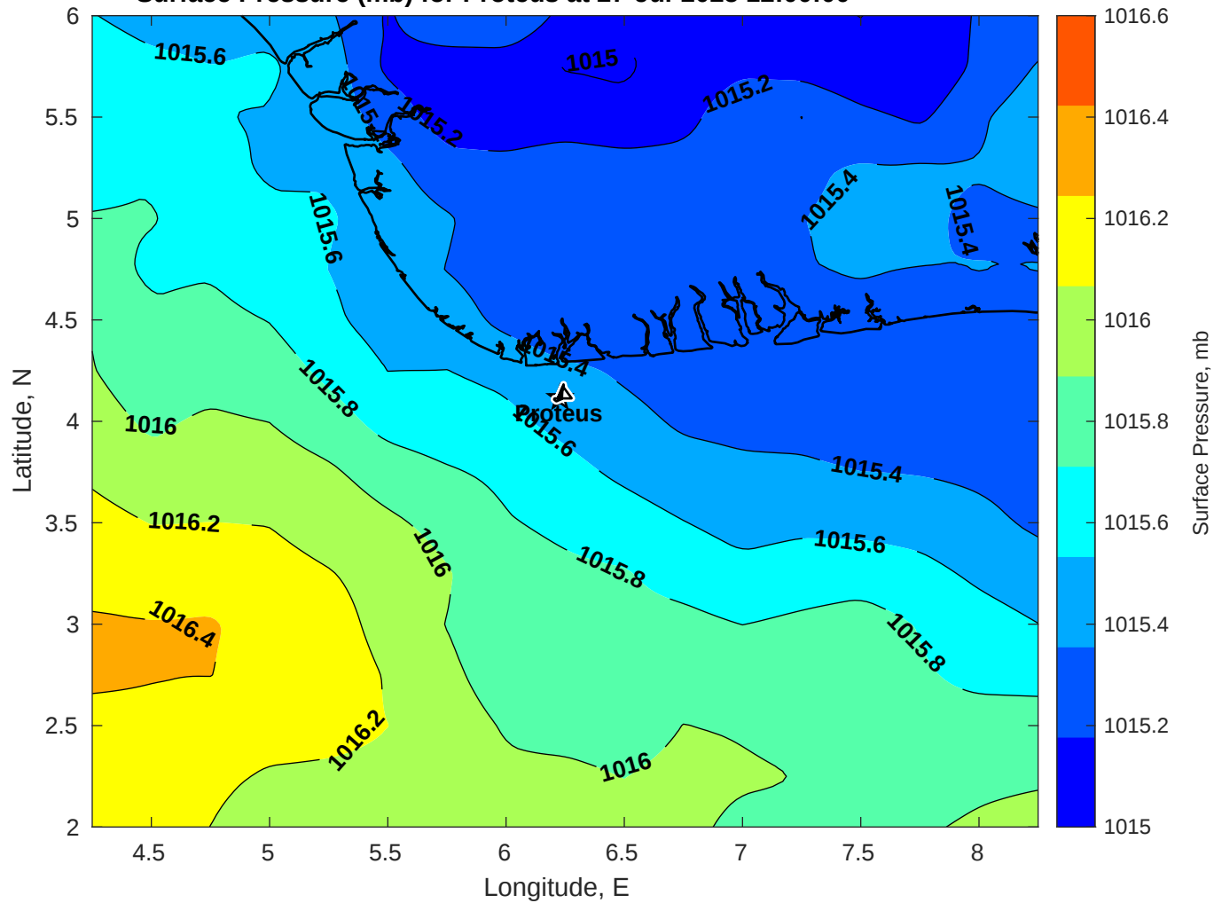
Surface Pressure (mb) for Proteus at 27-Jul-2025 12:00:00
