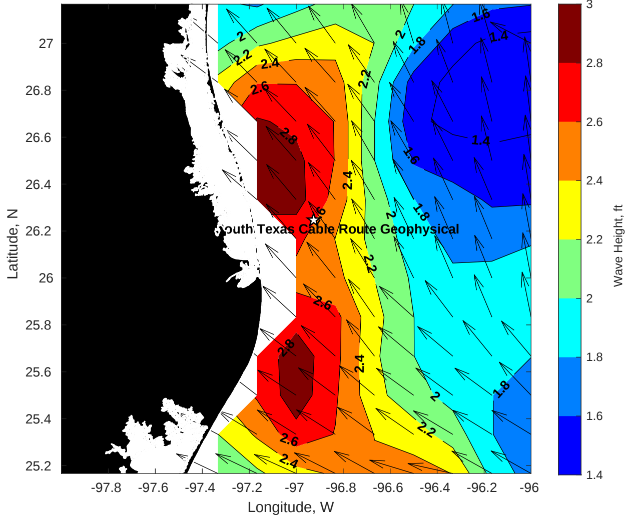
Wave Height (ft) for Tampnet P2378 South Texas Cable Route Geophysical at 25-Jul-2025 21:00:00
