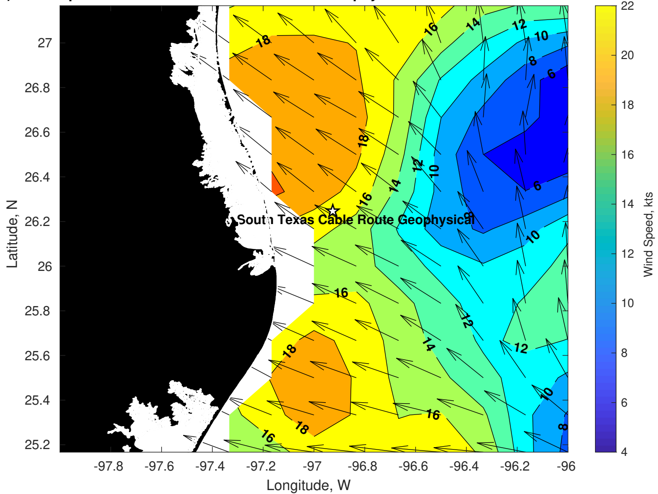
Winds (kts) for Tampnet P2378 South Texas Cable Route Geophysical at 25-Jul-2025 21:00:00
