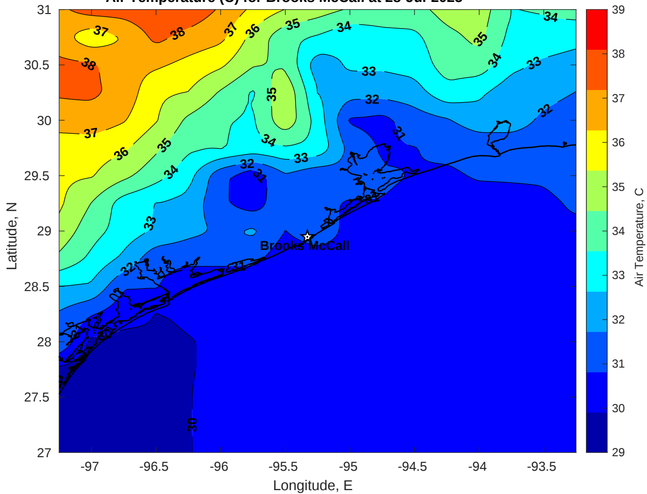
Air Temperature (C) for Brooks McCall at 28-Jul-2025
