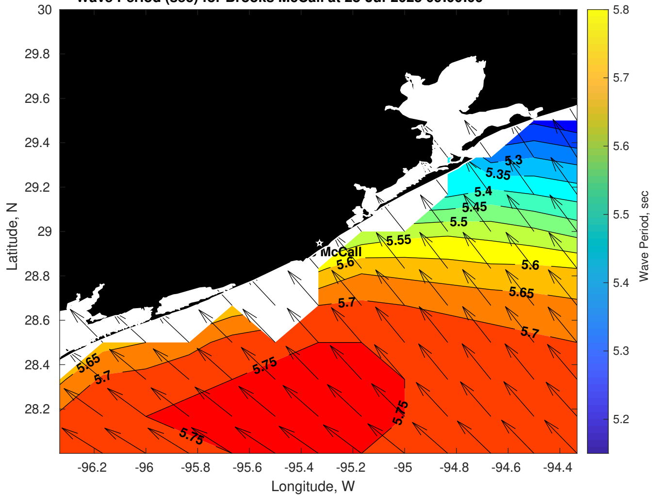
Wave Period (sec) for Brooks McCall at 28-Jul-2025 09:00:00
