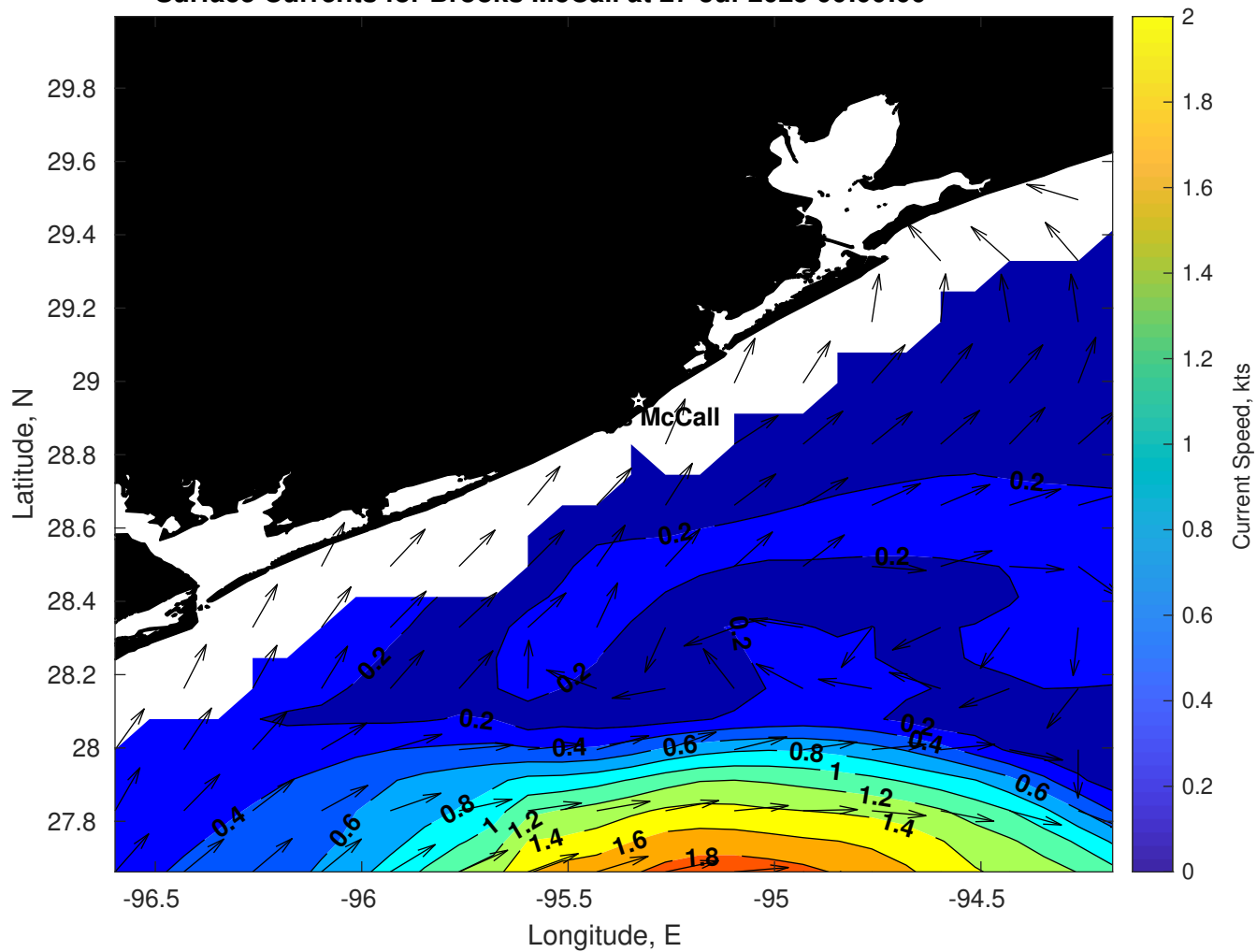
Surface Currents for Brooks McCall at 27-Jul-2025 00:00:00
