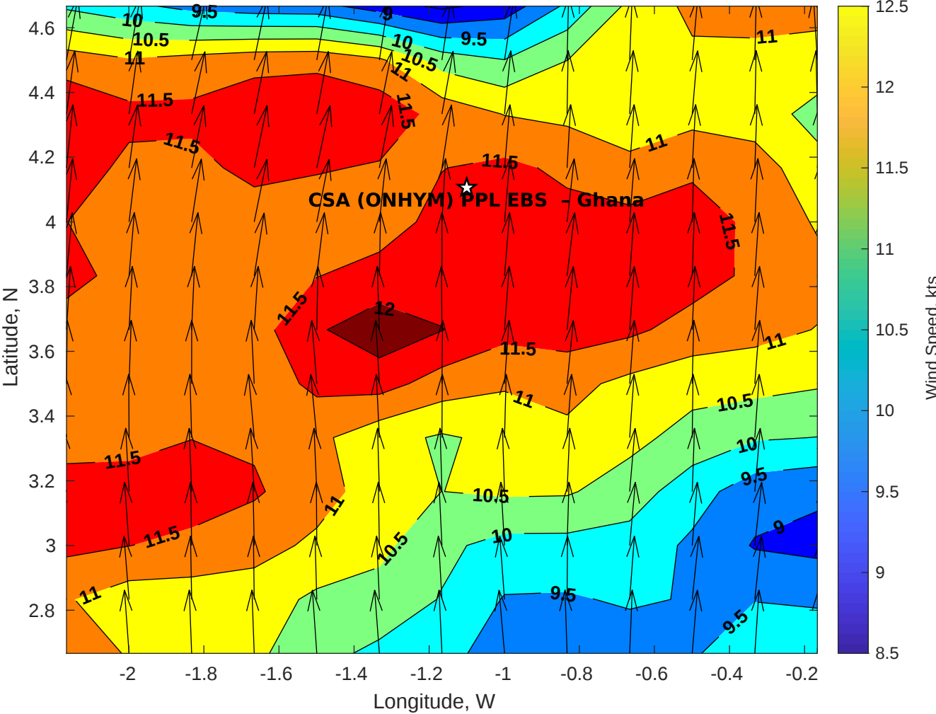
Winds (kts) for CSA (ONHYM) PPL EBS - Ghana at 28-Jul-2025 09:00:00
