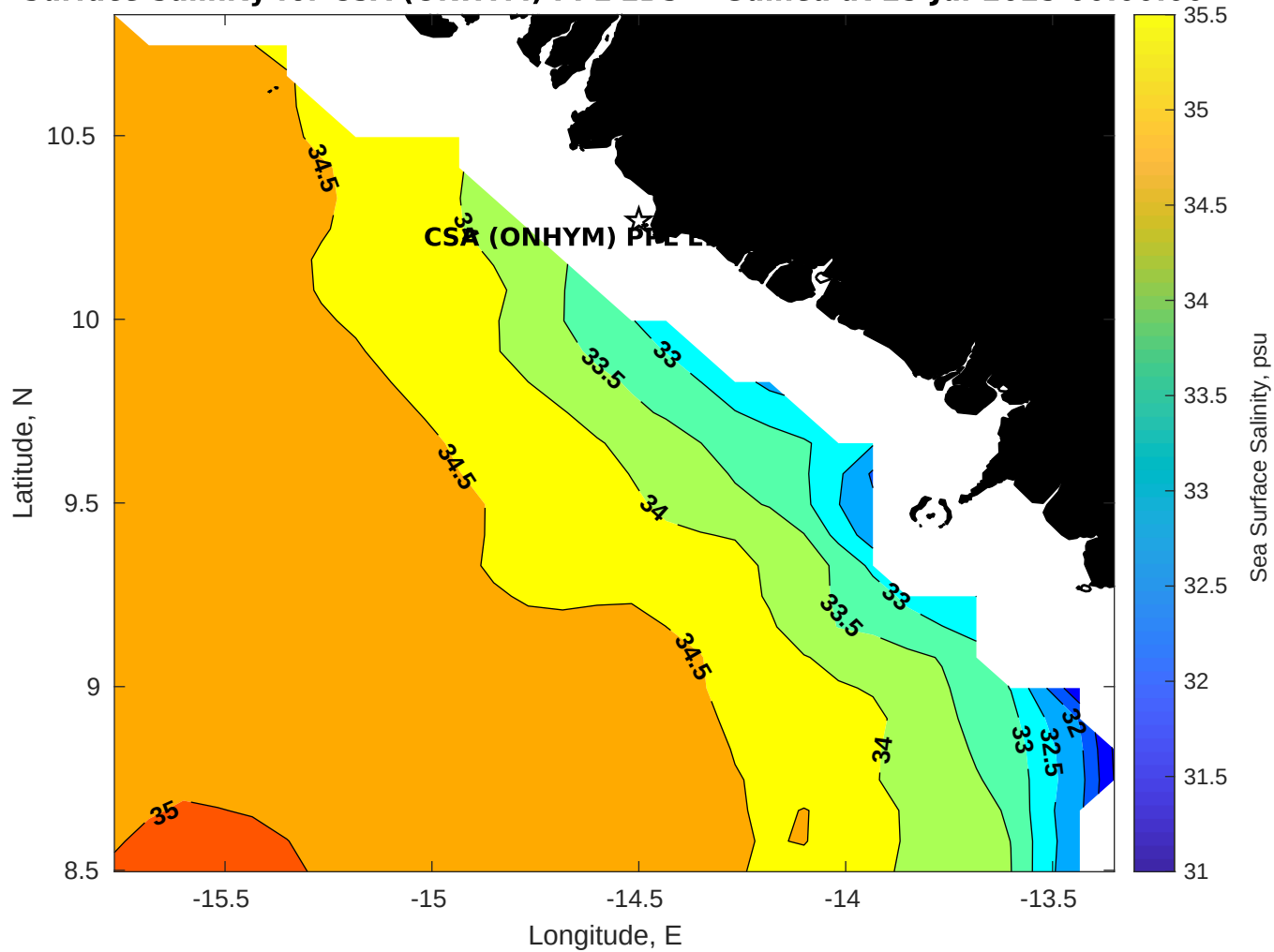
Surface Salinity for CSA (ONHYM) PPL EBS - Guinea at 25-Jul-2025 00:00:00
