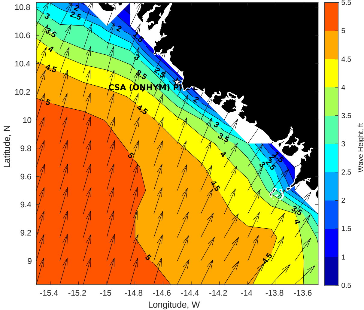
Wave Height (ft) for CSA (ONHYM) PPL EBS - Guinea at 28-Jul-2025 09:00:00
