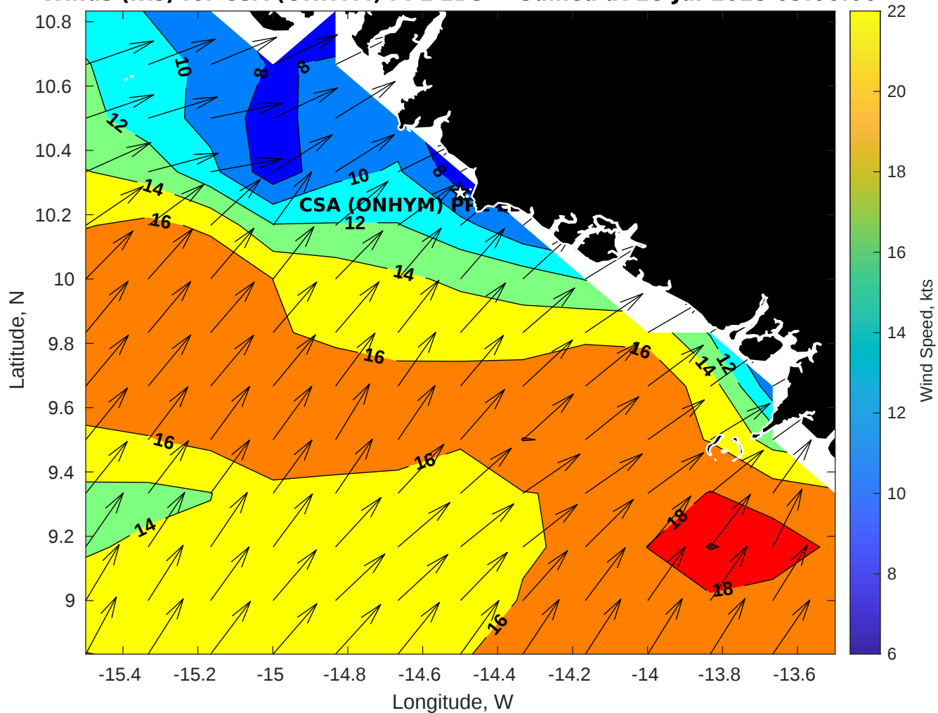
Winds (kts) for CSA (ONHYM) PPL EBS - Guinea at 28-Jul-2025 09:00:00
