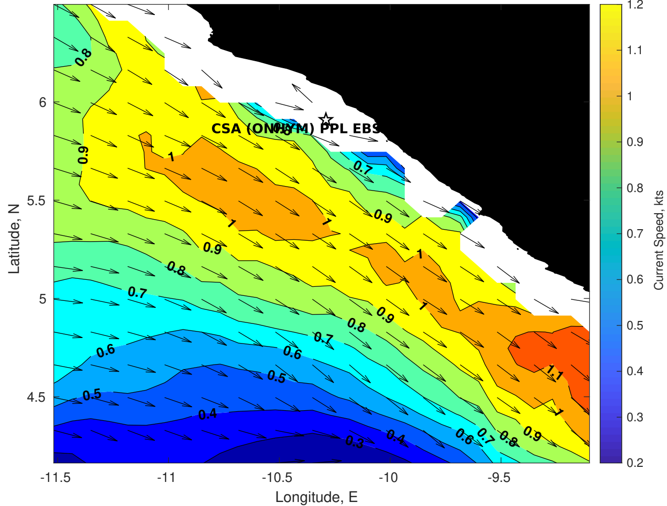
Surface Currents for CSA (ONHYM) PPL EBS - Liberia at 25-Jul-2025 00:00:00
