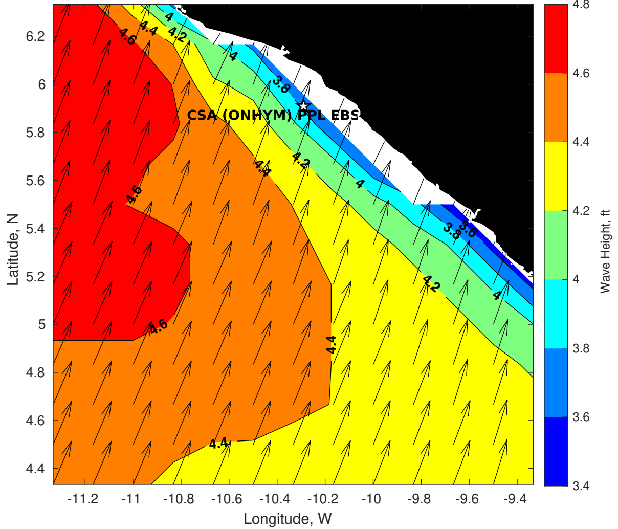
Wave Height (ft) for CSA (ONHYM) PPL EBS - Liberia at 28-Jul-2025 09:00:00
