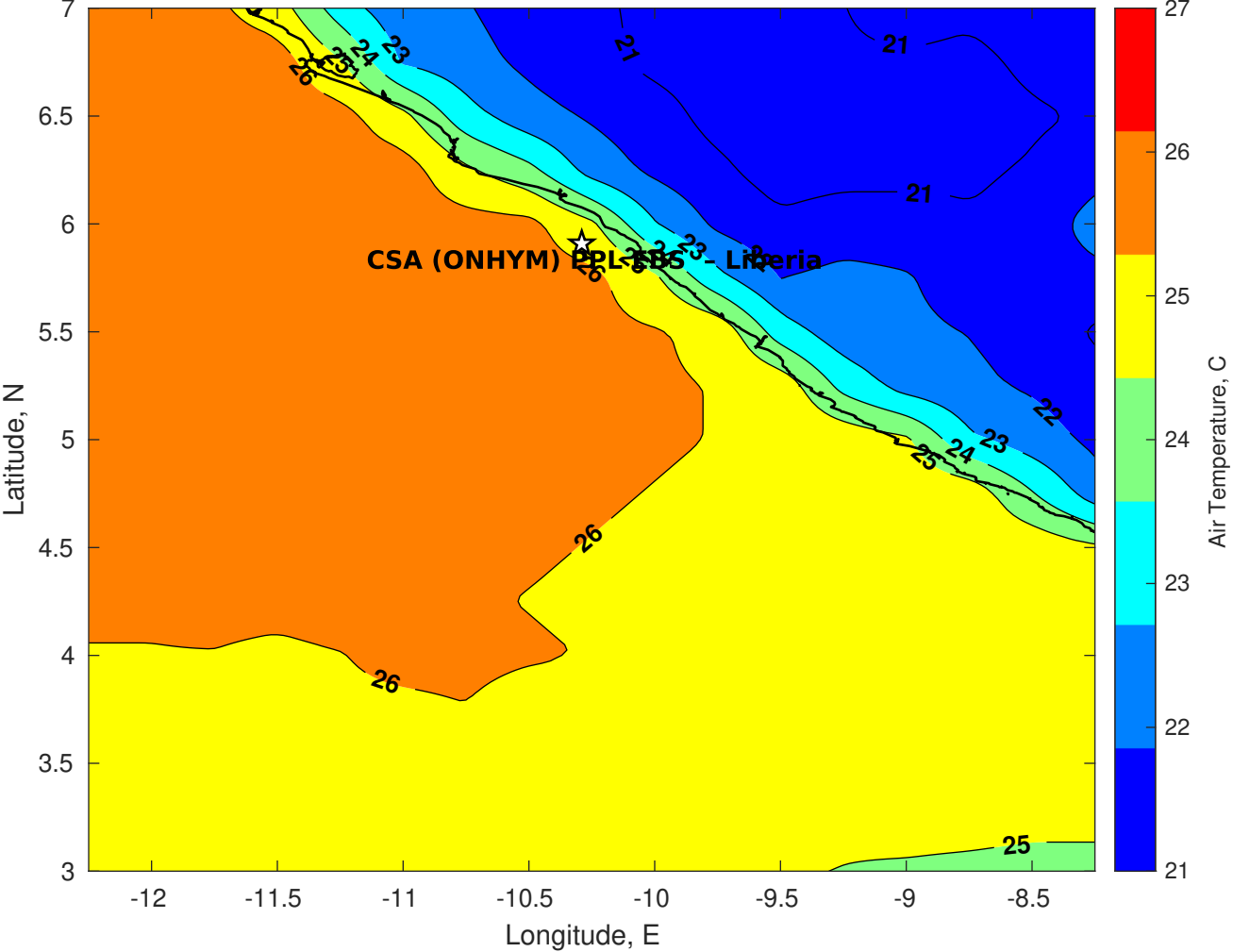
Air Temperature (C) for CSA (ONHYM) PPL EBS - Liberia at 28-Jul-2025
