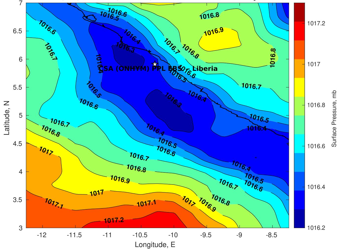
Surface Pressure (mb) for CSA (ONHYM) PPL EBS - Liberia at 30-Jul-2025 00:00:00
