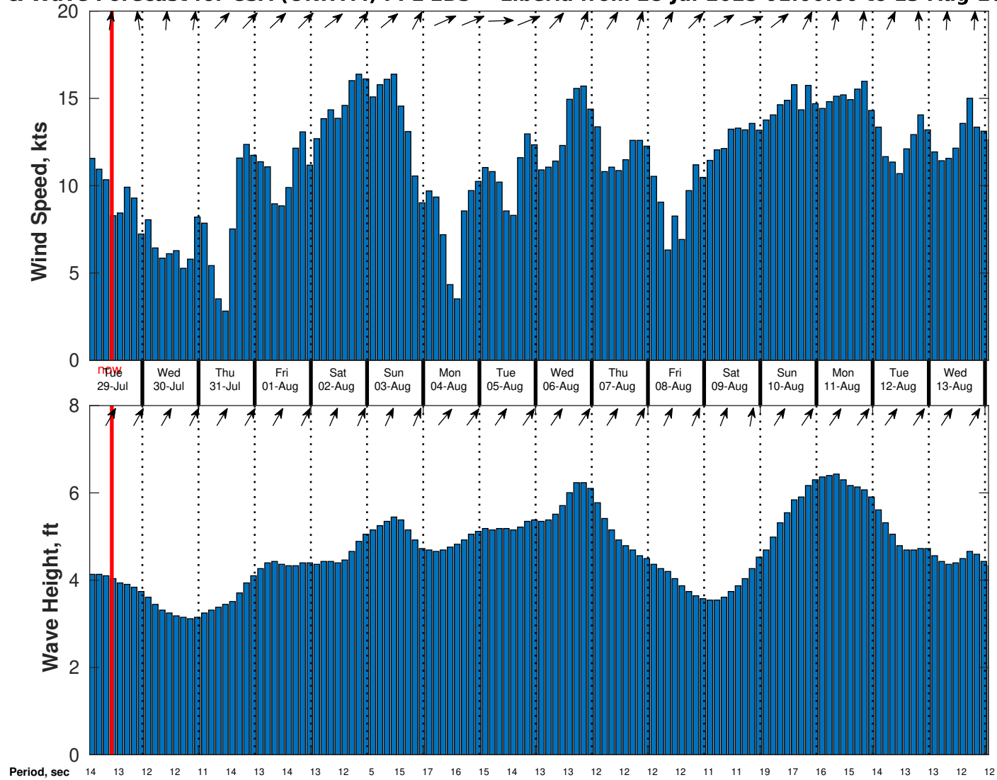
Wind & Wave Forecast for CSA (ONHYM) PPL EBS - Liberia from 28-Jul-2025 01:00:00 to 13-Aug-2025 01:00:00
