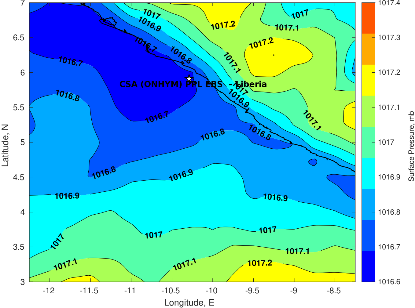
Surface Pressure (mb) for CSA (ONHYM) PPL EBS - Liberia at 29-Jul-2025 00:00:00
