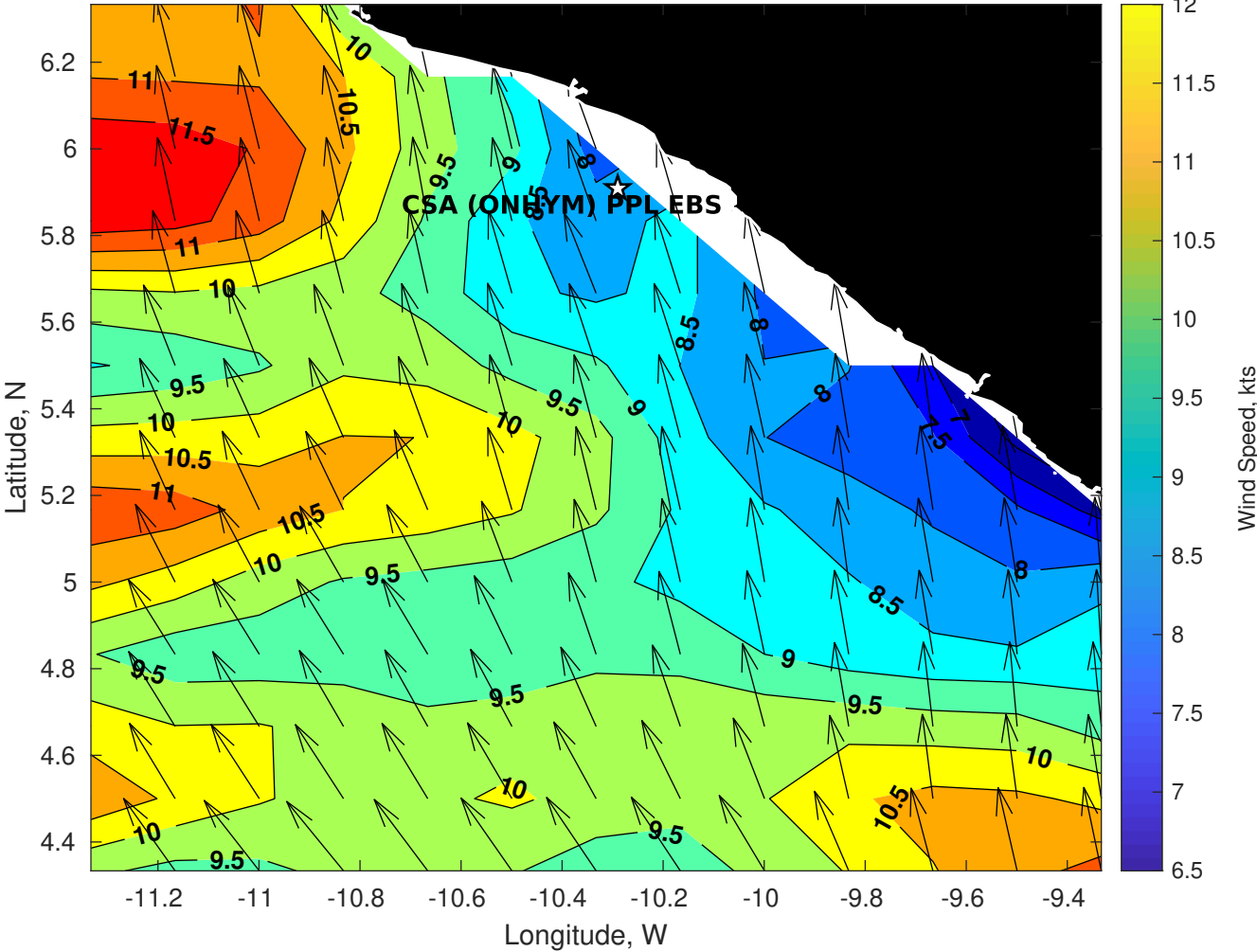
Winds (kts) for CSA (ONHYM) PPL EBS - Liberia at 28-Jul-2025 09:00:00
