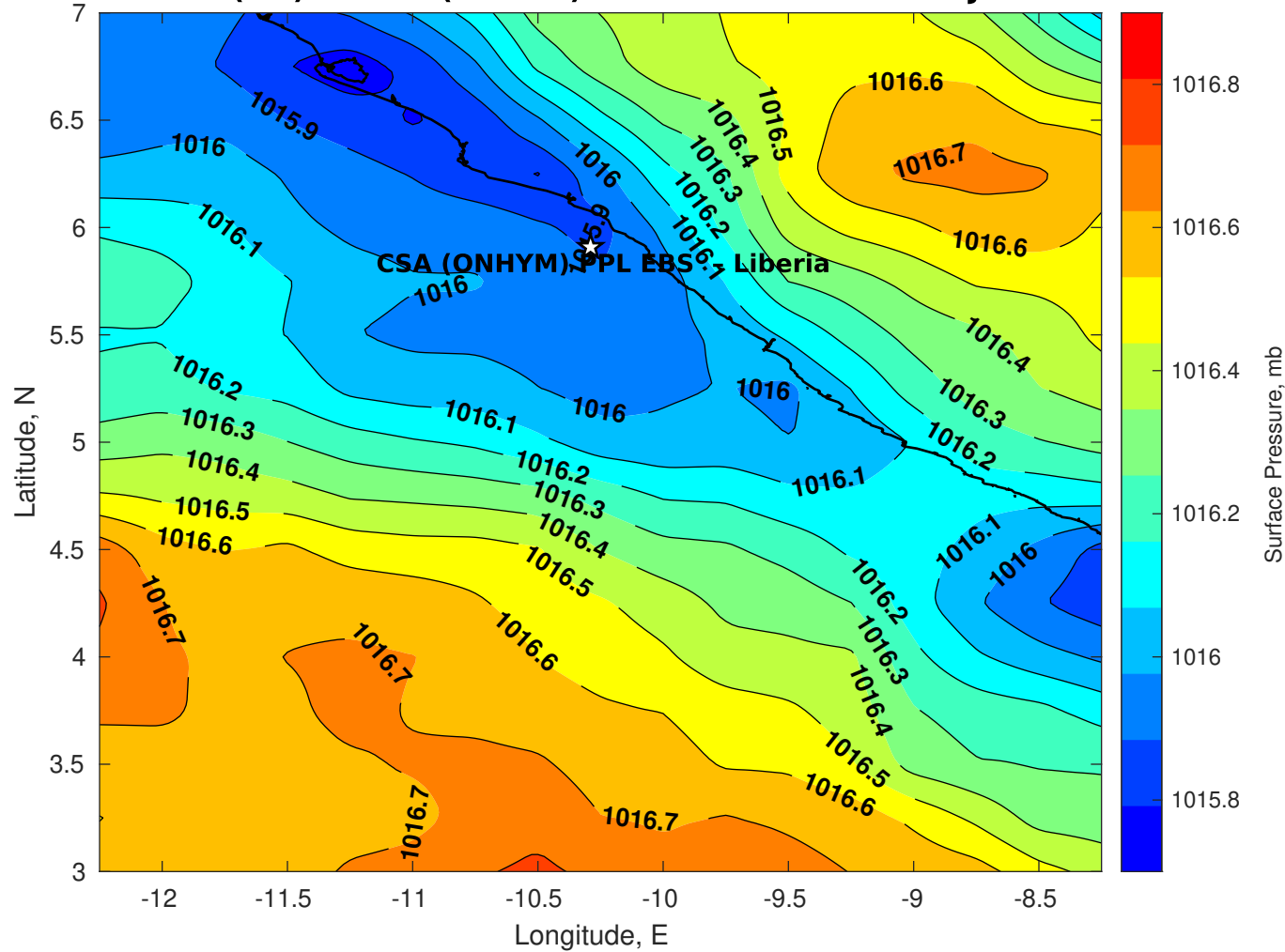
Surface Pressure (mb) for CSA (ONHYM) PPL EBS - Liberia at 28-Jul-2025 00:00:00
