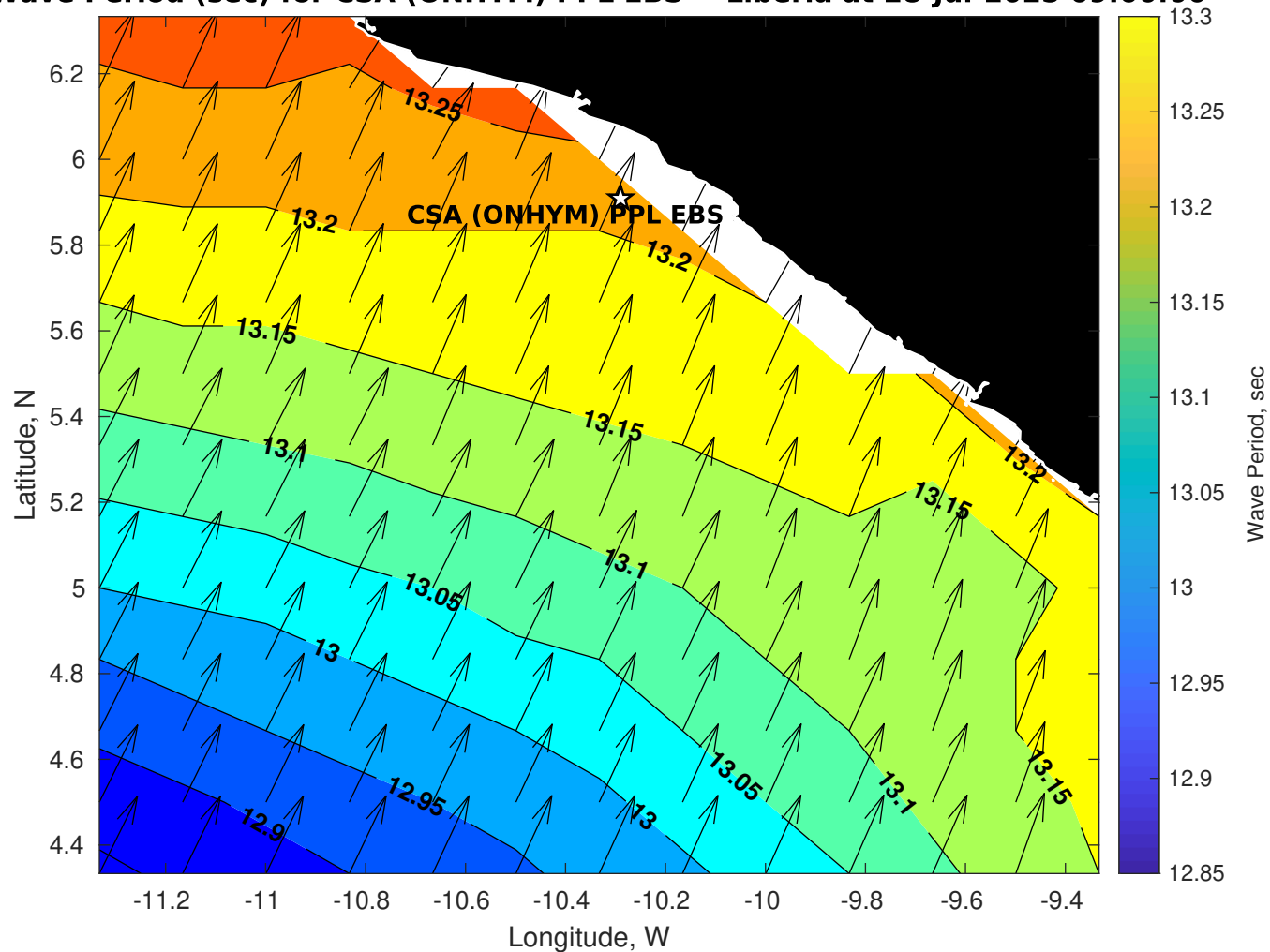
Wave Period (sec) for CSA (ONHYM) PPL EBS - Liberia at 28-Jul-2025 09:00:00
