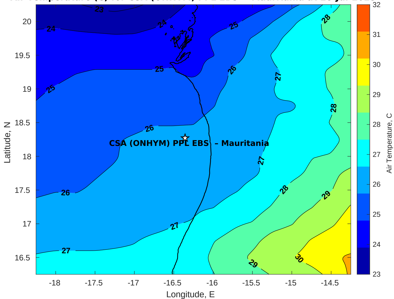
Air Temperature (C) for CSA (ONHYM) PPL EBS - Mauritania at 28-Jul-2025
