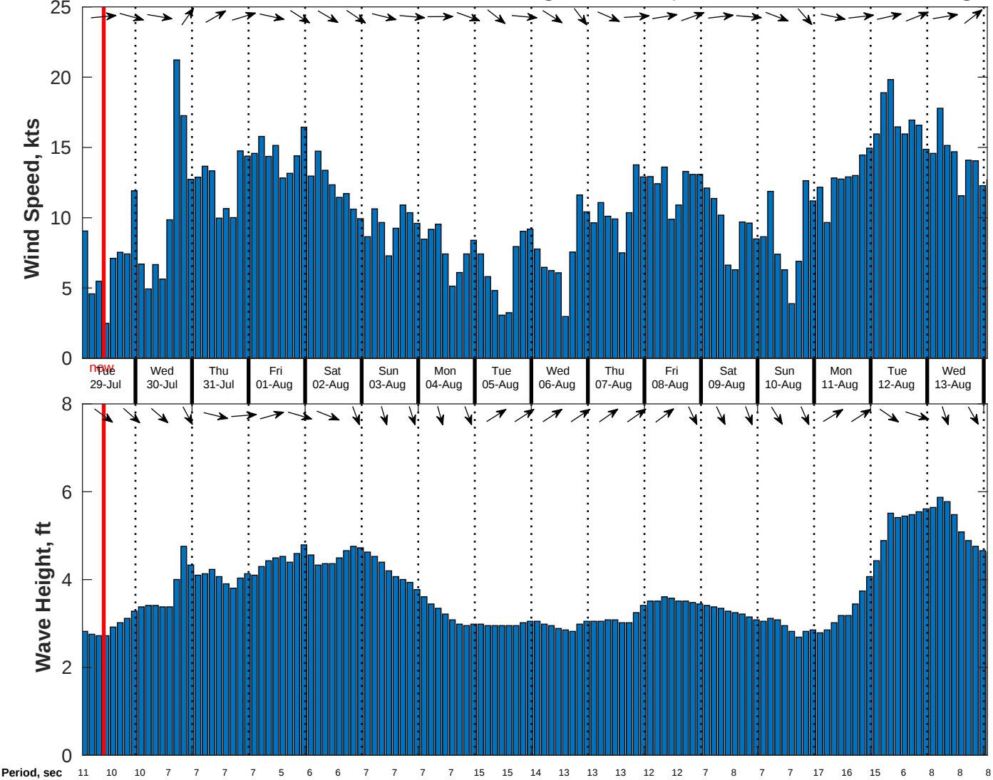
Wind & Wave Forecast for CSA (ONHYM) PPL EBS - Senegal from 28-Jul-2025 01:00:00 to 13-Aug-2025 01:00:00
