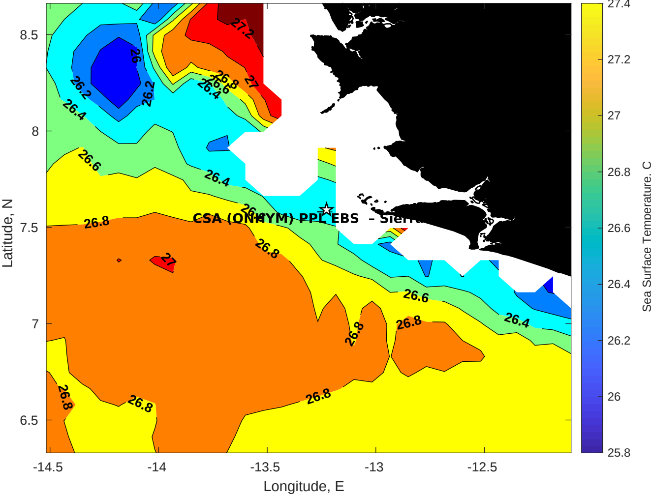
SST for CSA (ONHYM) PPL EBS - Sierra Leone at 25-Jul-2025 00:00:00
