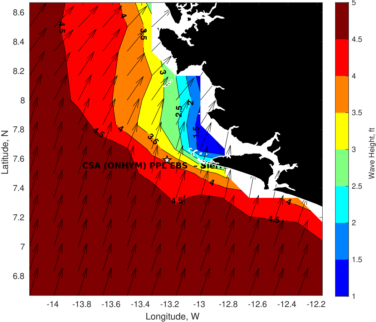
Wave Height (ft) for CSA (ONHYM) PPL EBS - Sierra Leone at 28-Jul-2025 09:00:00
