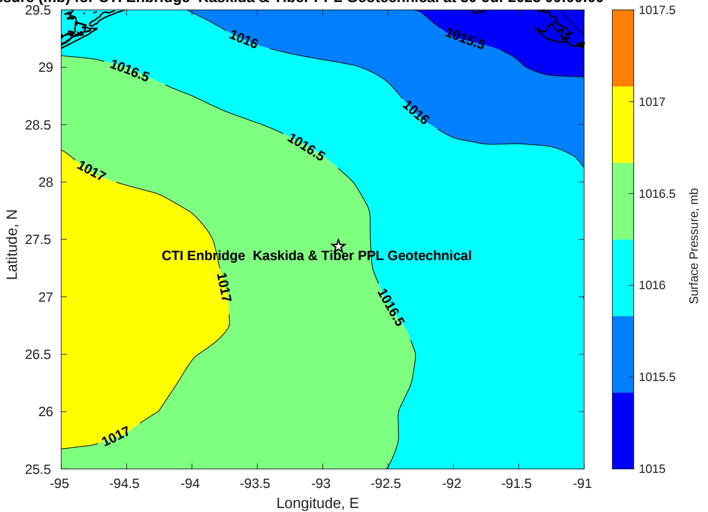
Surface Pressure (mb) for CTI Enbridge Kaskida & Tiber PPL Geotechnical at 30-Jul-2025 00:00:00
