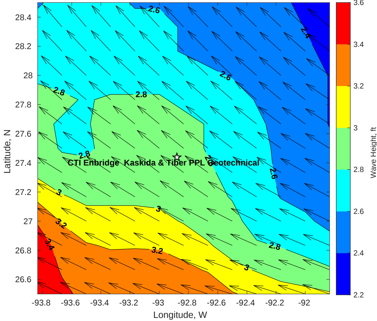
Wave Height (ft) for CTI Enbridge Kaskida & Tiber PPL Geotechnical at 28-Jul-2025 09:00:00
