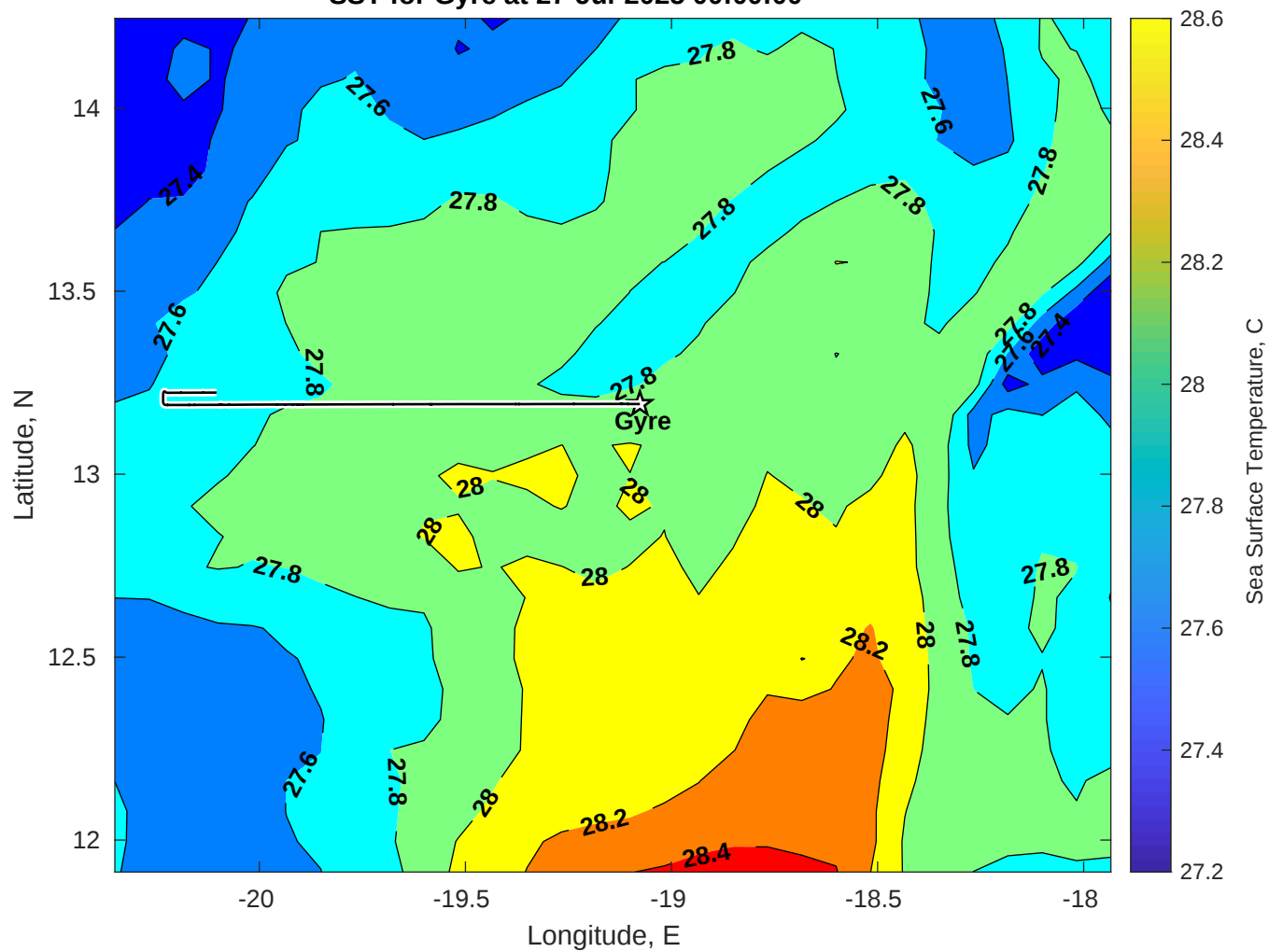
SST for Gyre at 27-Jul-2025 00:00:00
