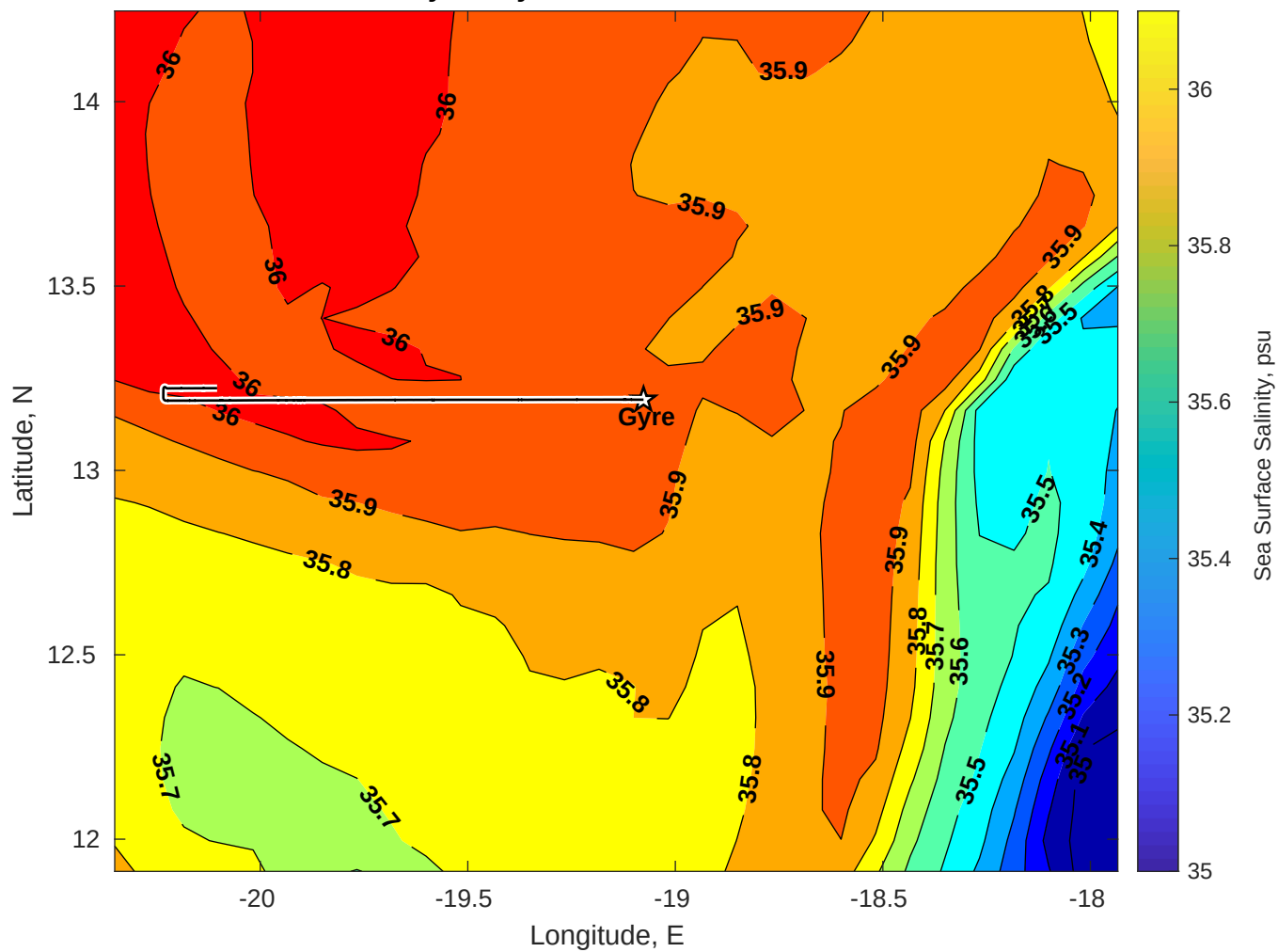
Surface Salinity for Gyre at 27-Jul-2025 00:00:00
