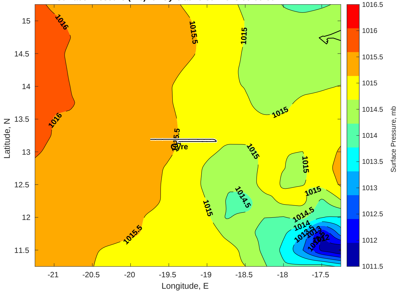
Surface Pressure (mb) for Gyre at 29-Jul-2025 00:00:00
