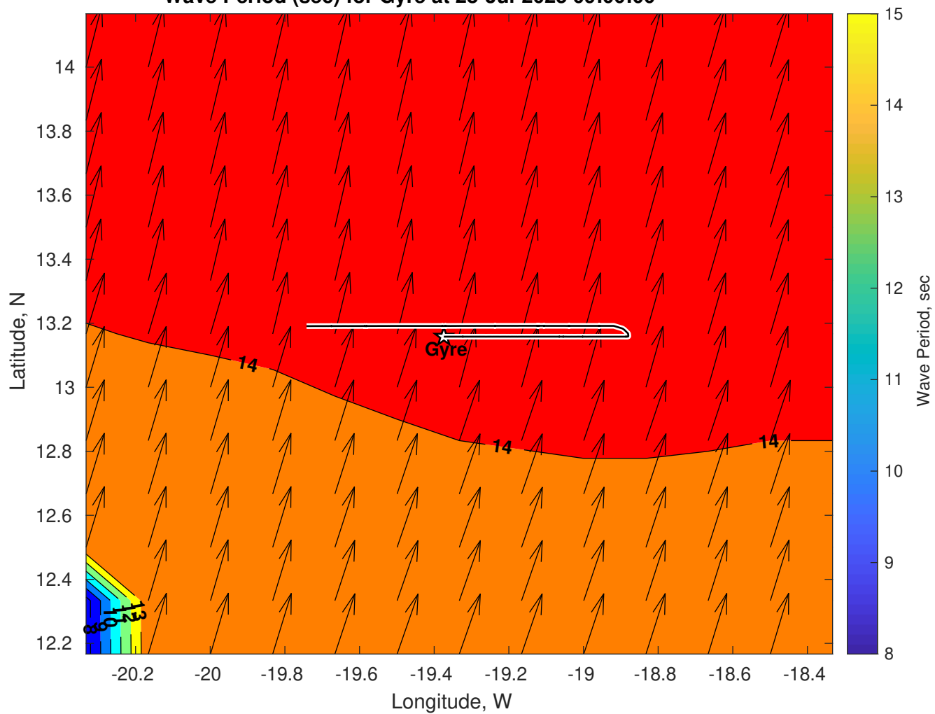
Wave Period (sec) for Gyre at 28-Jul-2025 09:00:00
