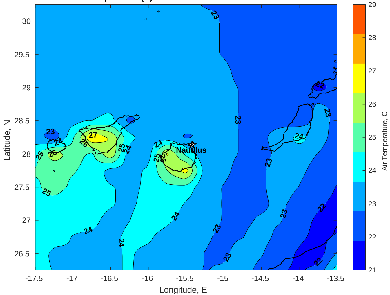
Air Temperature (C) for Nautilus at 28-Jul-2025
