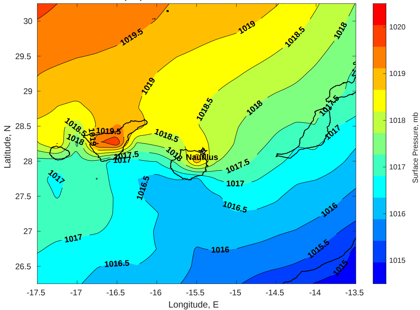
Surface Pressure (mb) for Nautilus at 29-Jul-2025 00:00:00
