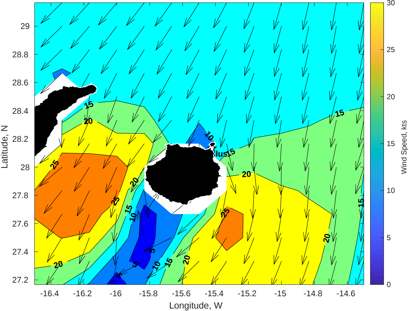
Winds (kts) for Nautilus at 28-Jul-2025 09:00:00
