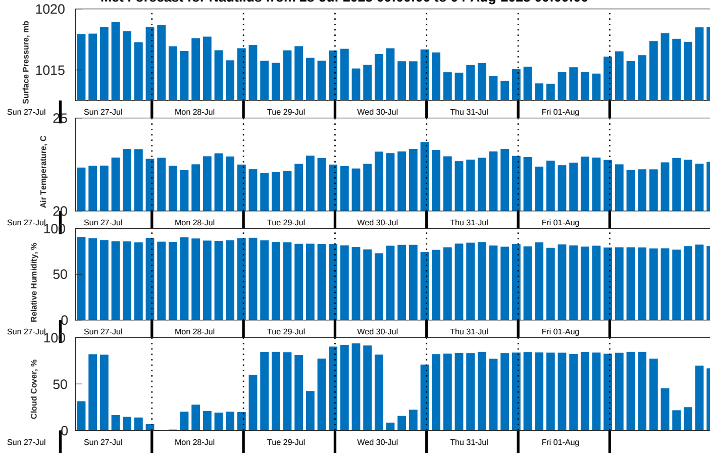
Met Forecast for Nautilus from 28-Jul-2025 00:00:00 to 04-Aug-2025 00:00:00
