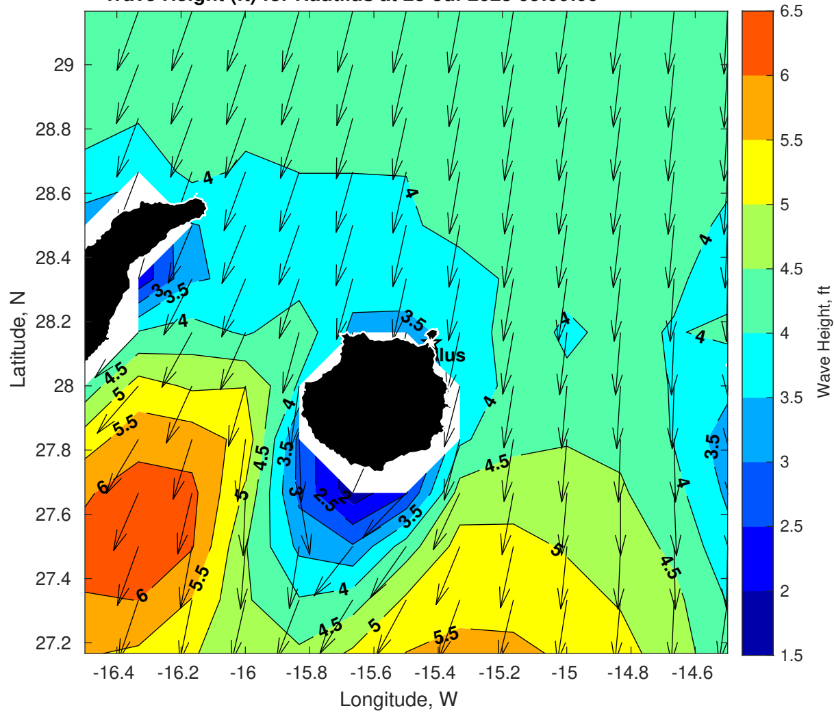
Wave Height (ft) for Nautilus at 28-Jul-2025 09:00:00
