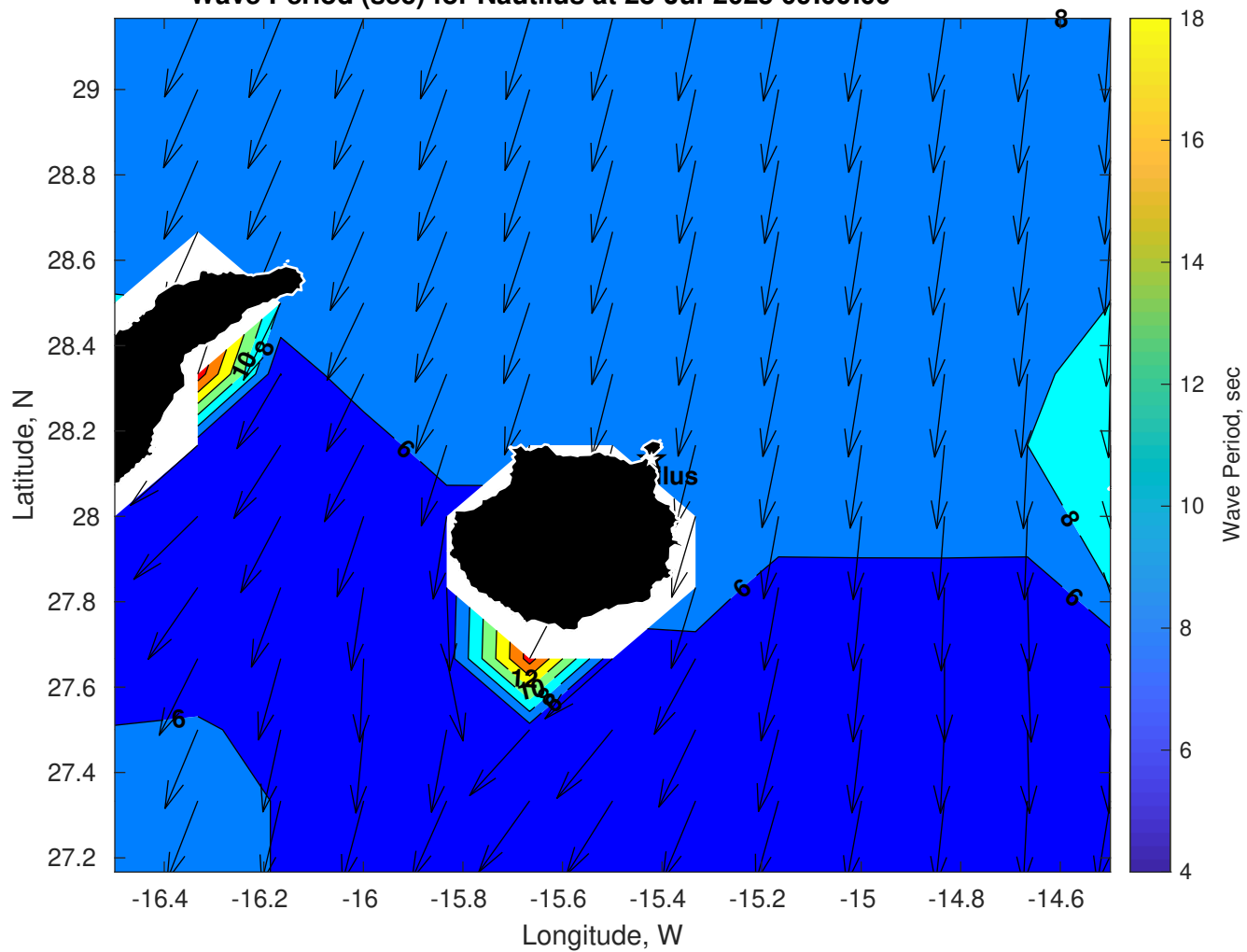
Wave Period (sec) for Nautilus at 28-Jul-2025 09:00:00
