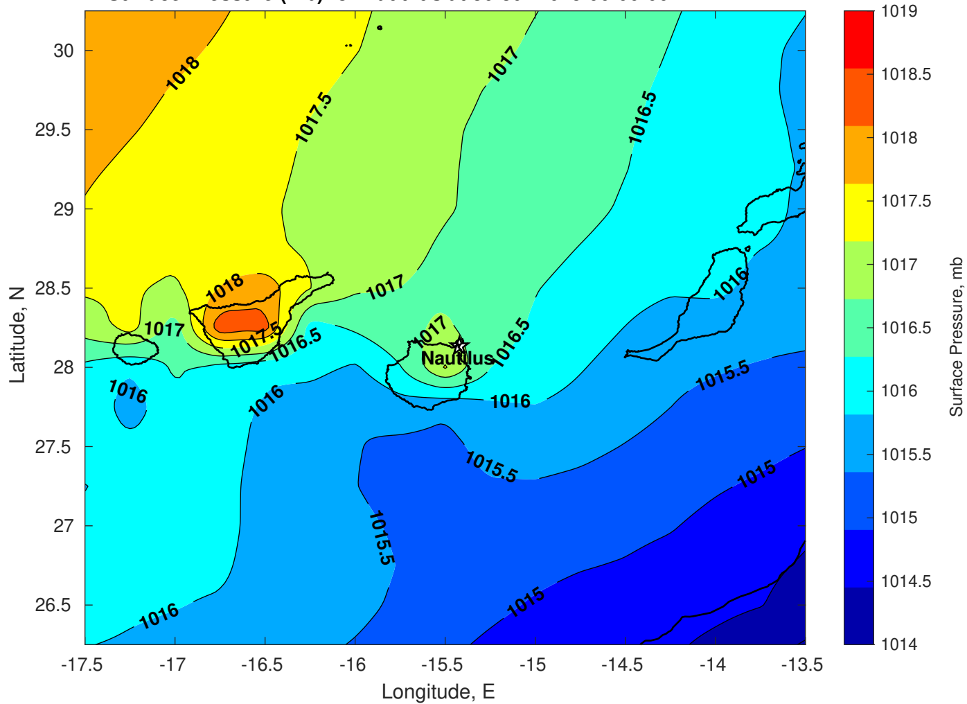
Surface Pressure (mb) for Nautilus at 30-Jul-2025 00:00:00
