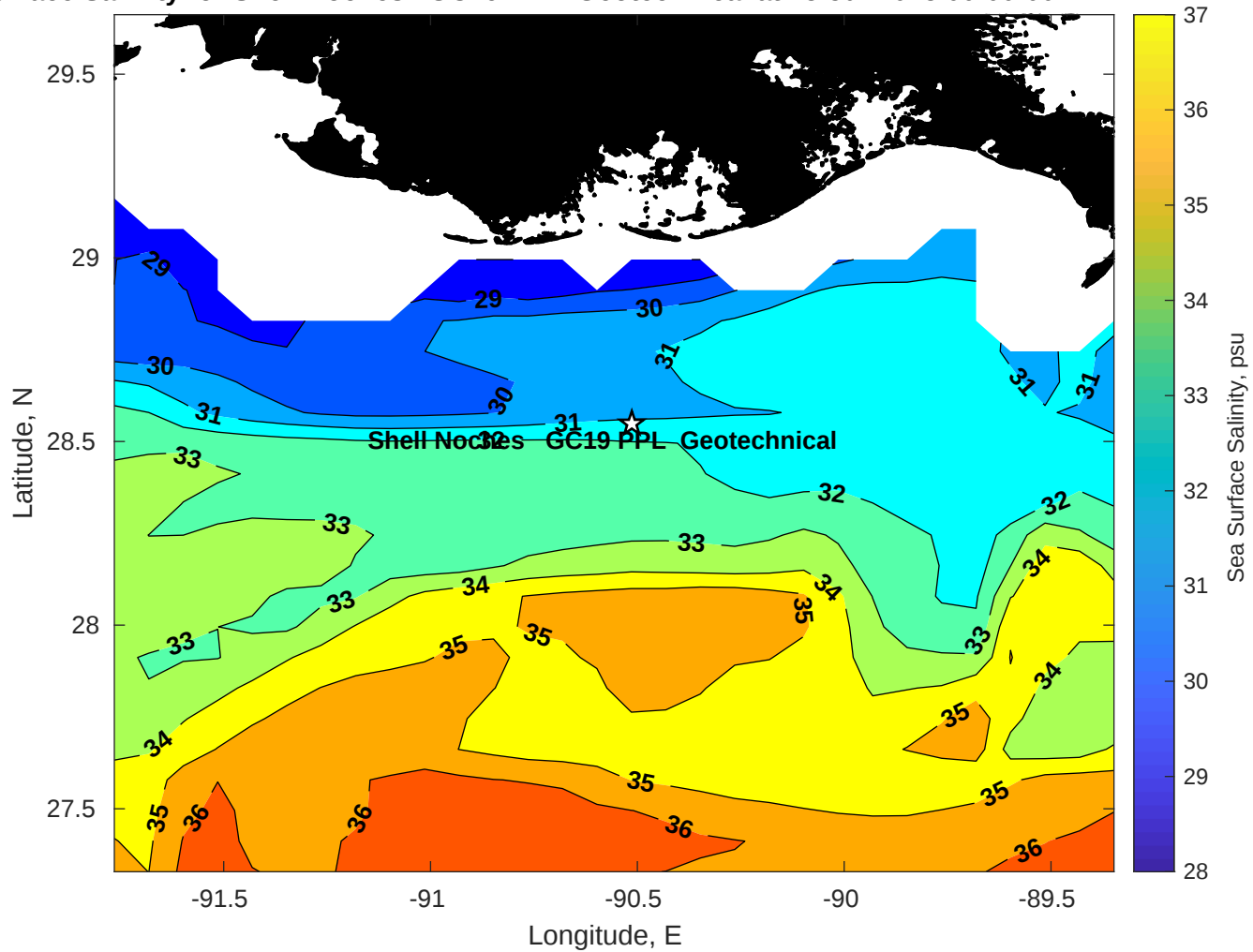
Surface Salinity for Shell Noches GC19 PPL Geotechnical at 25-Jul-2025 00:00:00
