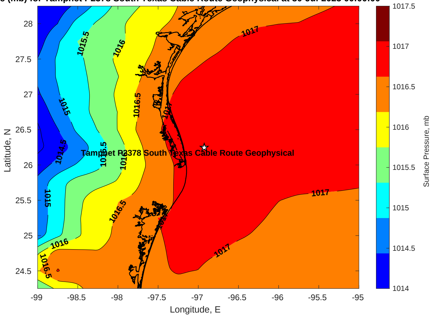
Pressure (mb) for Tampnet P2378 South Texas Cable Route Geophysical at 30-Jul-2025 00:00:00
