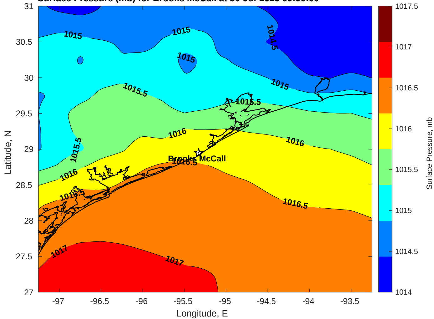
Surface Pressure (mb) for Brooks McCall at 30-Jul-2025 00:00:00
