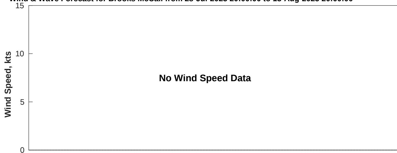
Wind & Wave Forecast for Brooks McCall from 28-Jul-2025 20:00:00 to 13-Aug-2025 20:00:00
