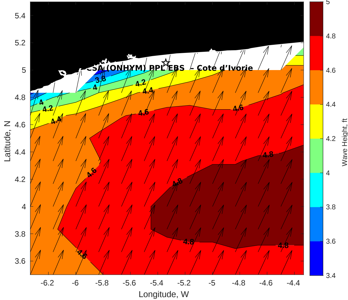
Wave Height (ft) for CSA (ONHYM) PPL EBS - Cote d'Ivoire at 28-Jul-2025 09:00:00
