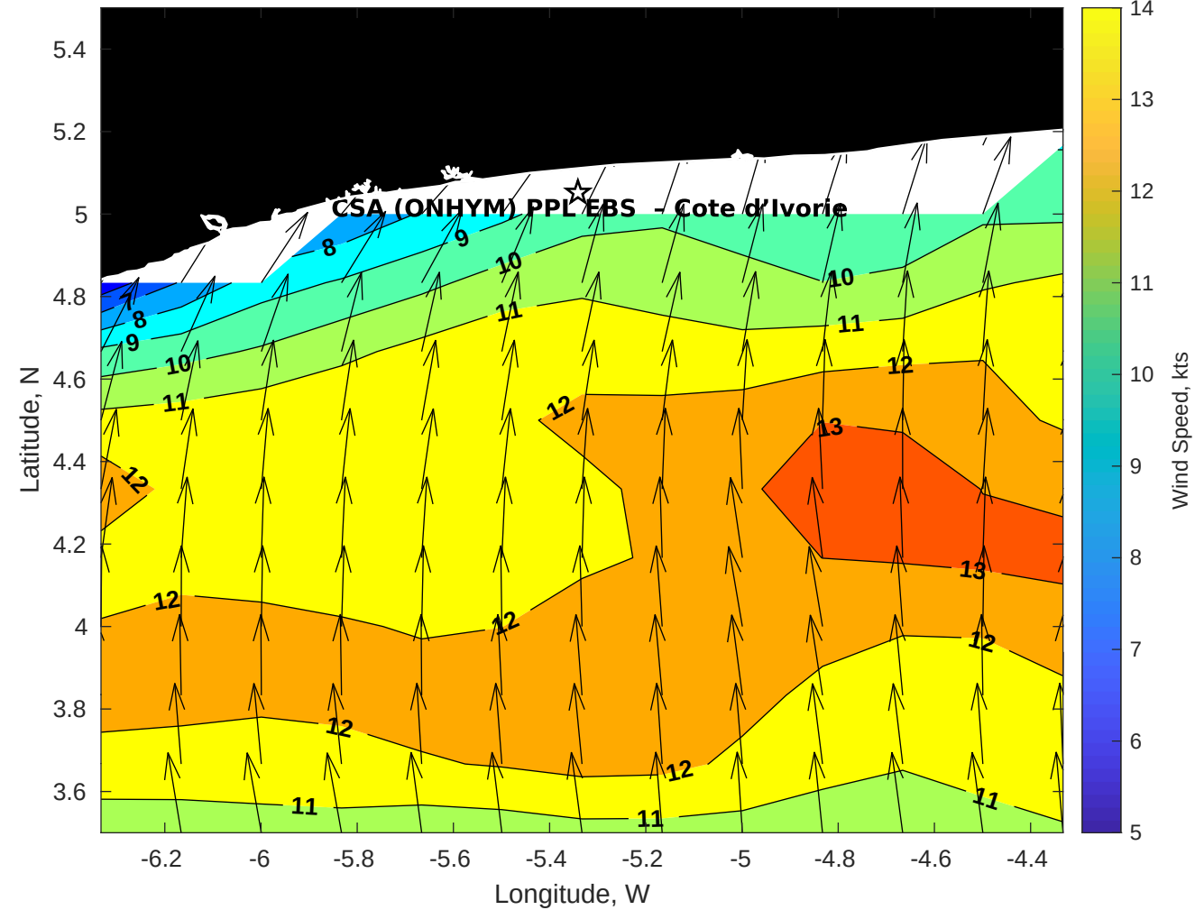
Winds (kts) for CSA (ONHYM) PPL EBS - Cote d'Ivoire at 28-Jul-2025 09:00:00
