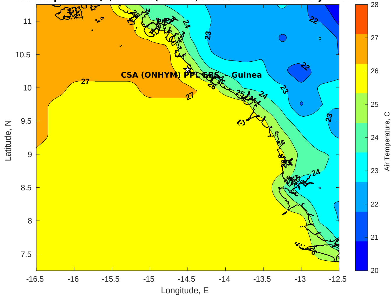
Air Temperature (C) for CSA (ONHYM) PPL EBS - Guinea at 28-Jul-2025
