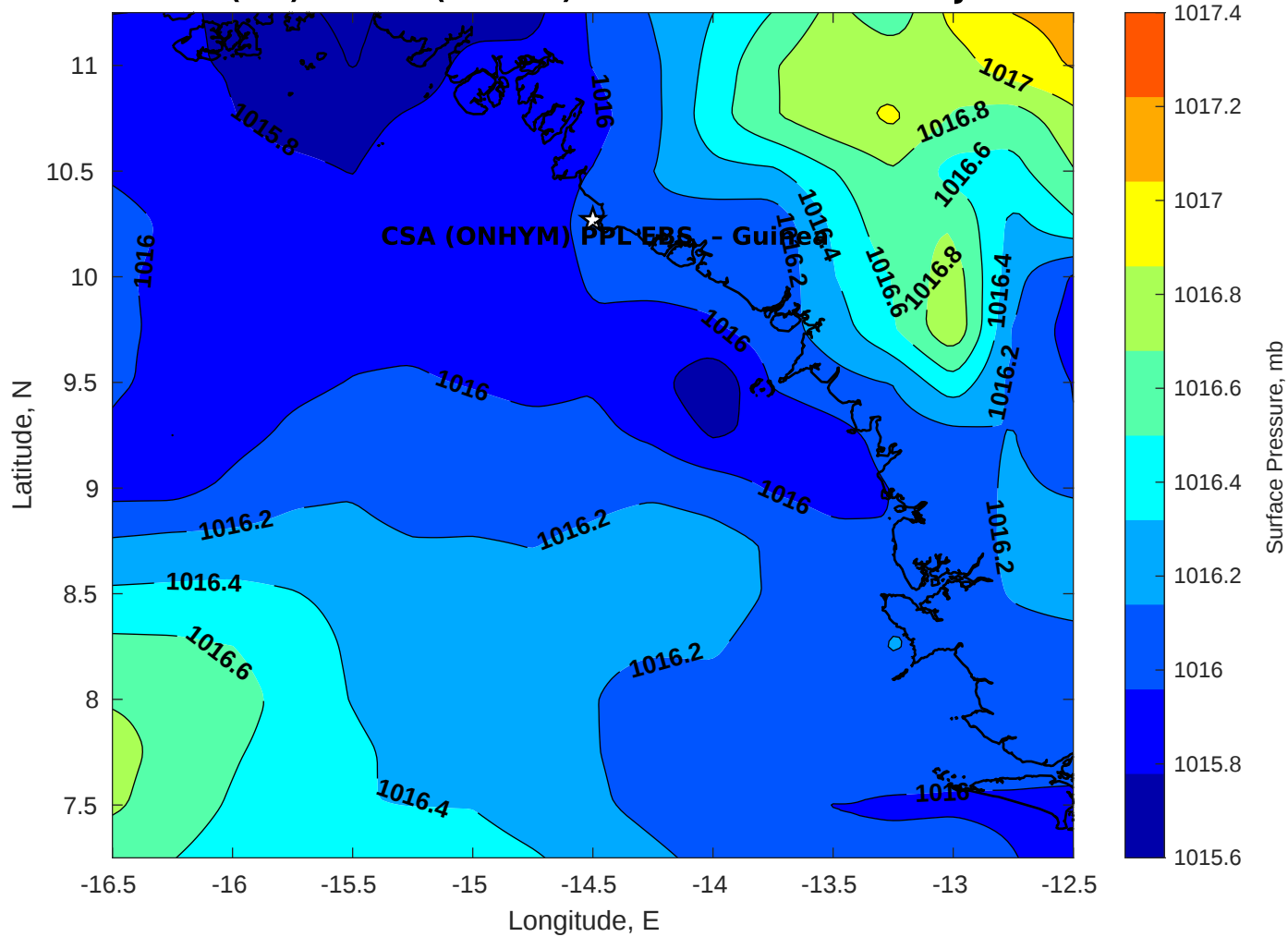
Surface Pressure (mb) for CSA (ONHYM) PPL EBS - Guinea at 28-Jul-2025 00:00:00
