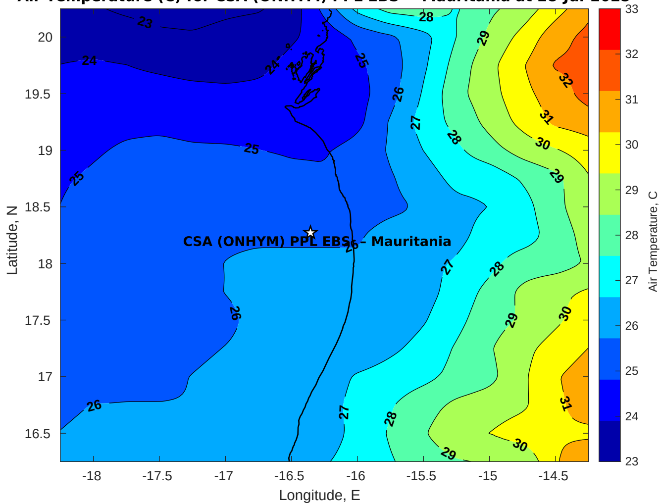
Air Temperature (C) for CSA (ONHYM) PPL EBS - Mauritania at 28-Jul-2025
