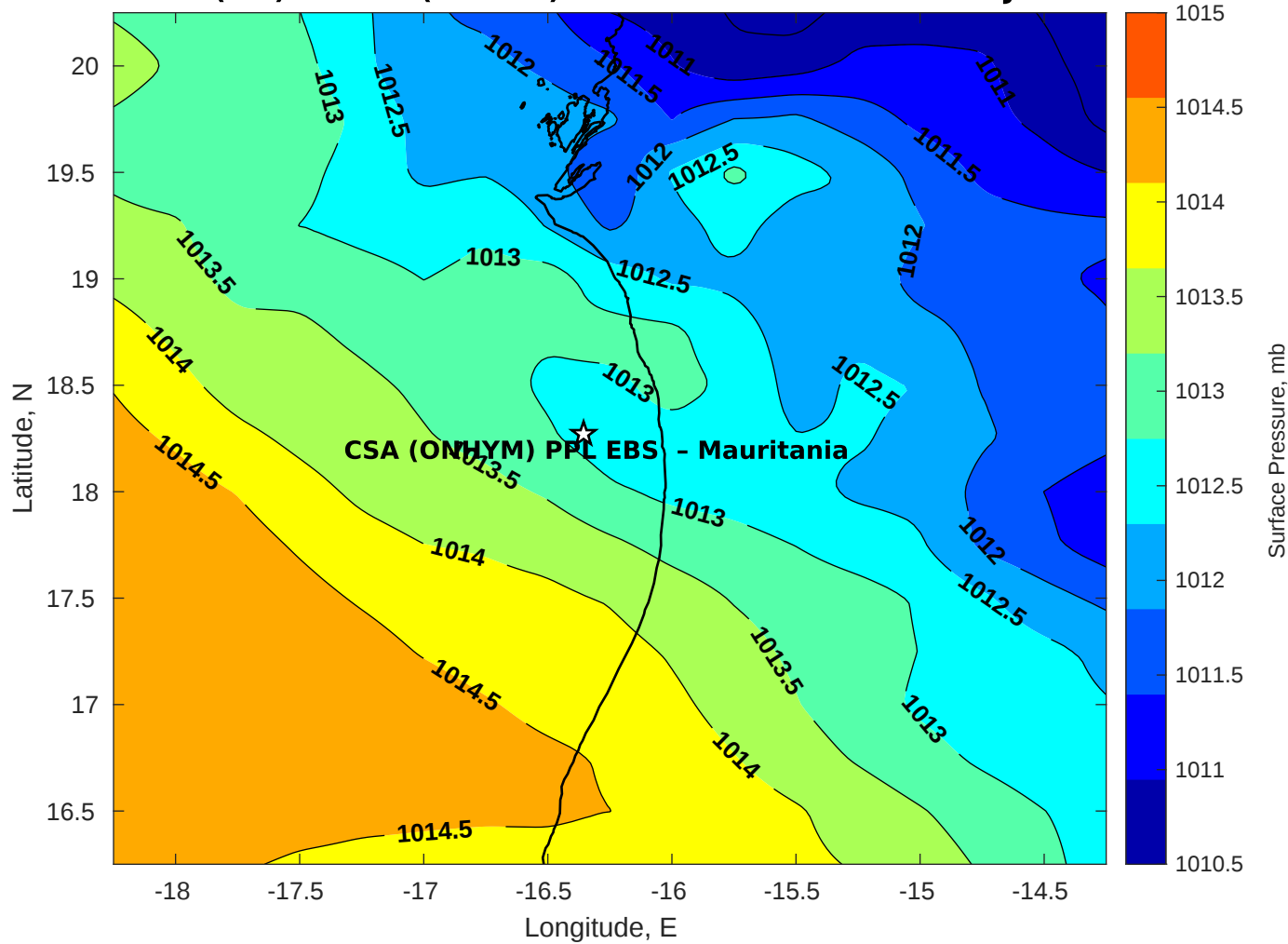
Surface Pressure (mb) for CSA (ONHYM) PPL EBS - Mauritania at 29-Jul-2025 00:00:00
