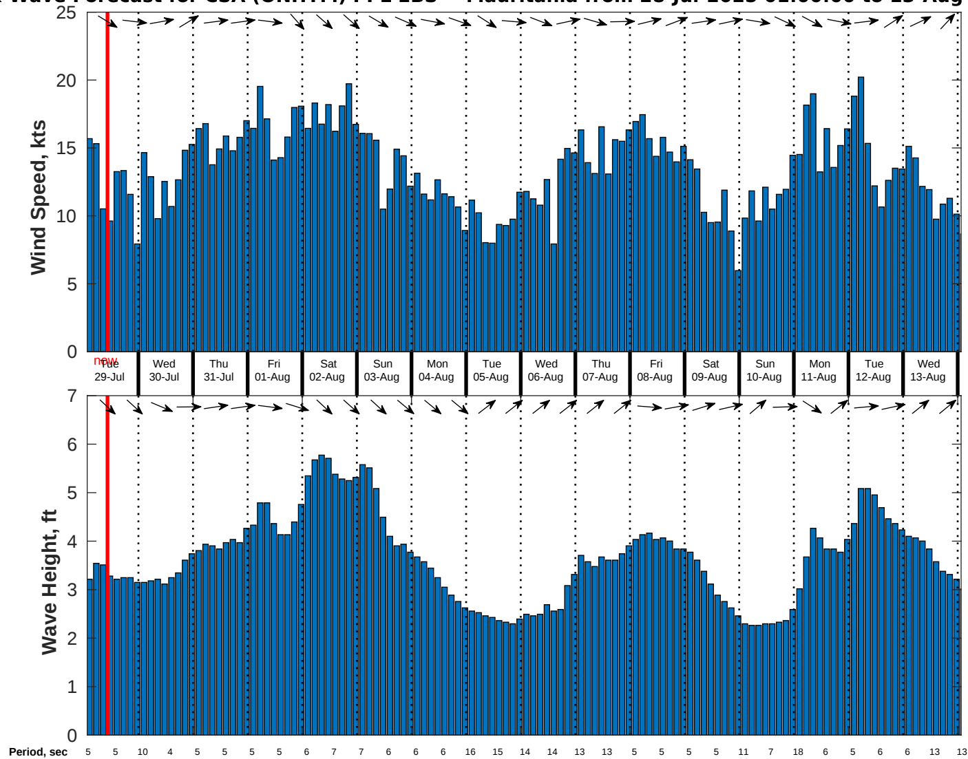
Wind & Wave Forecast for CSA (ONHYM) PPL EBS - Mauritania from 28-Jul-2025 01:00:00 to 13-Aug-2025 01:00:00
