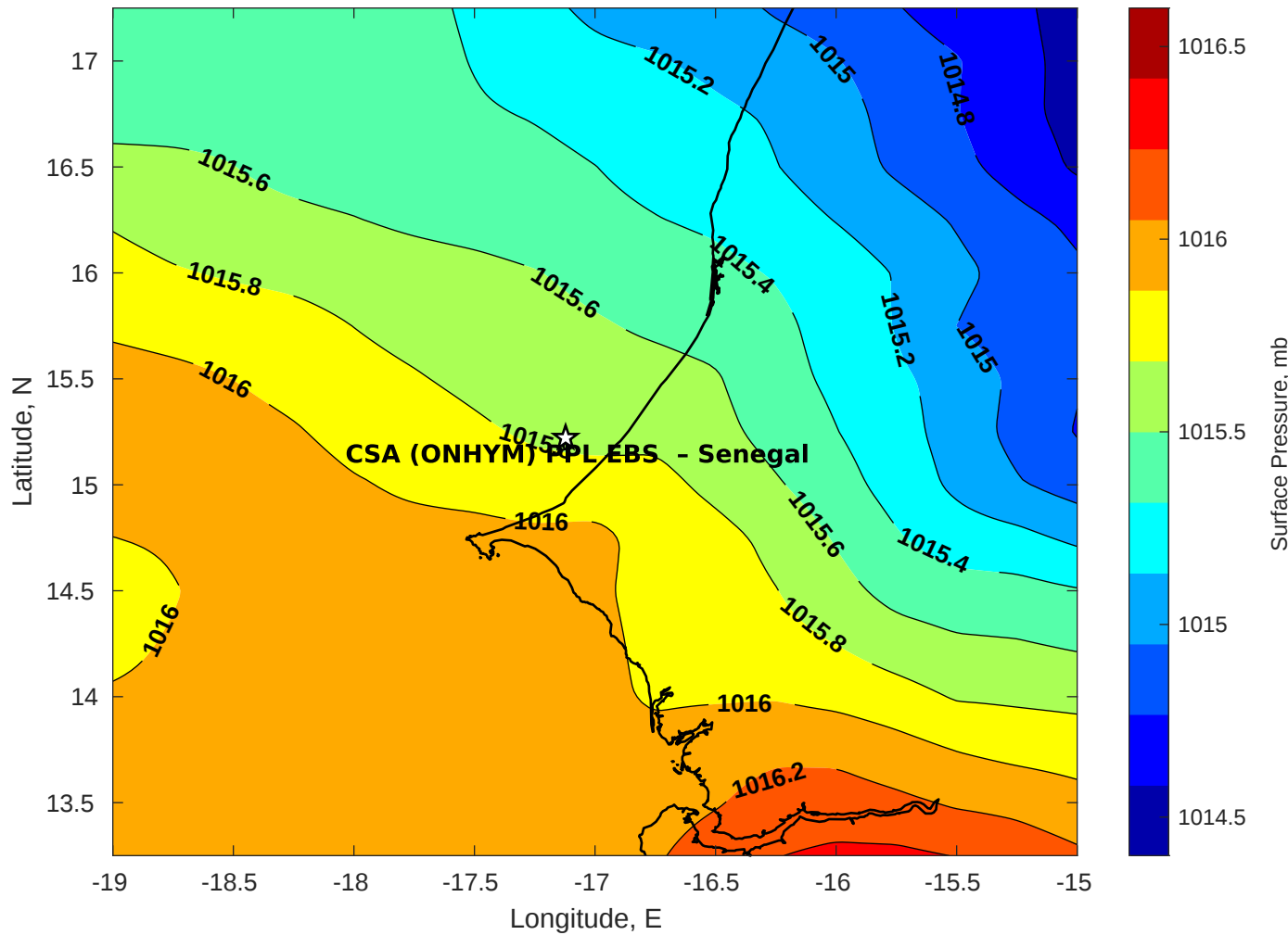
Surface Pressure (mb) for CSA (ONHYM) PPL EBS - Senegal at 30-Jul-2025 00:00:00
